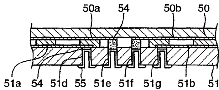
FIG.9 (PRIOR ART)
