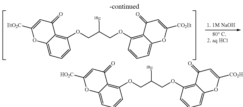
5,5'-(2-[18F]fluoropropane-1,3-diyl)bis(oxy)bis(4-oxo-4H-chromene-2-carboxylic acid)
