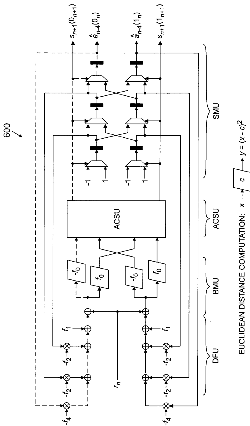
FIG. 6 (PRIOR ART)
