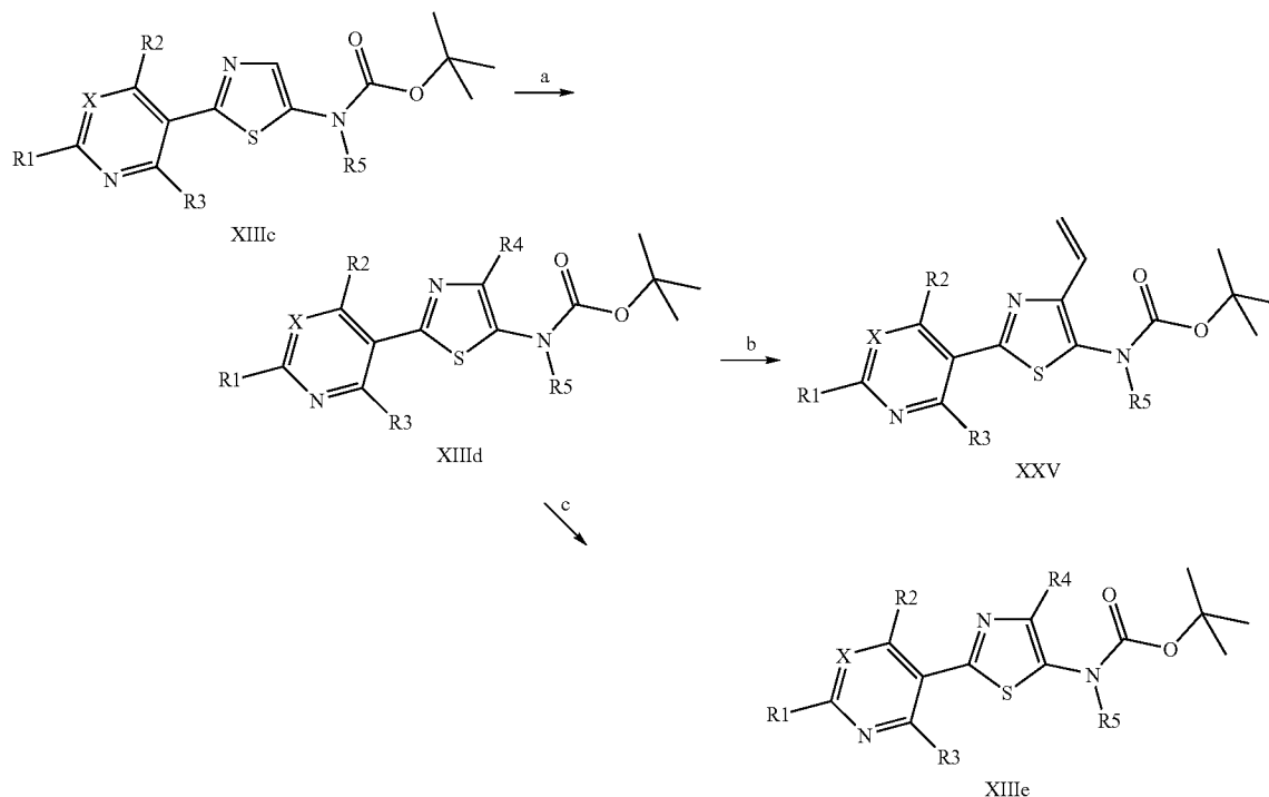
Scheme IX
