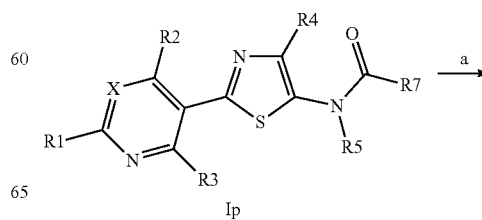
Scheme XIII
