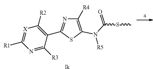
Scheme XI
