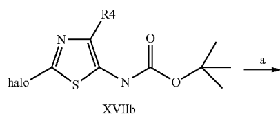
Scheme X
