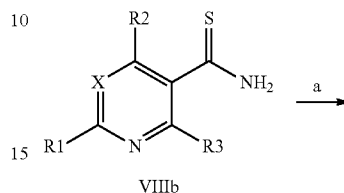
Scheme XII
