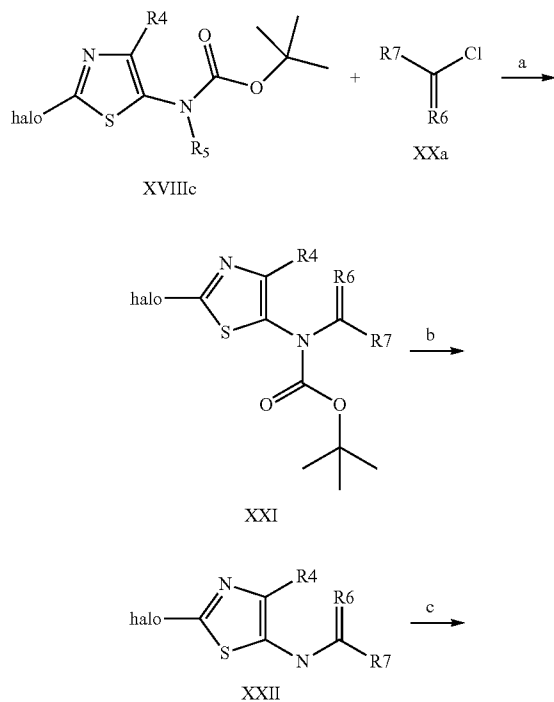
Scheme IV
