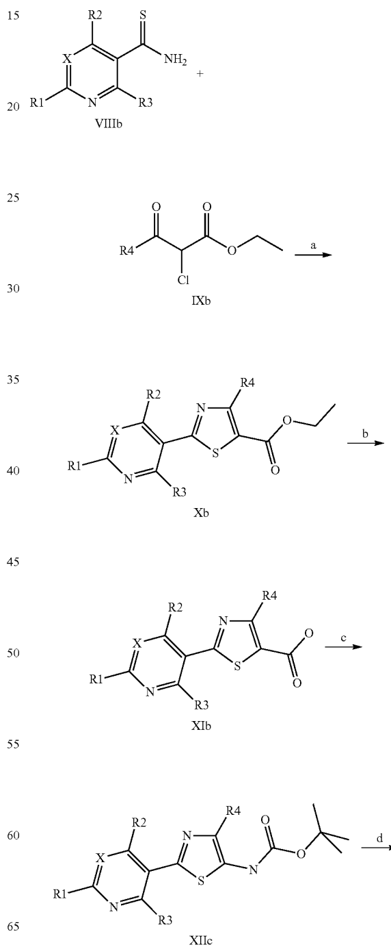
Scheme XVII
