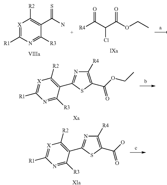
Scheme II
