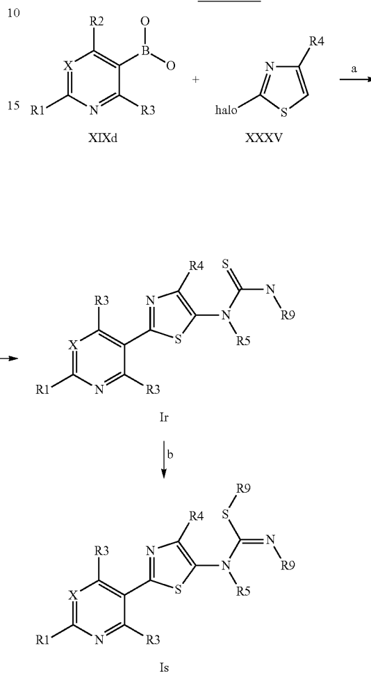
Scheme XV
