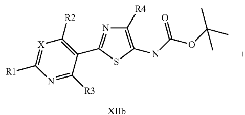
Scheme VIII
