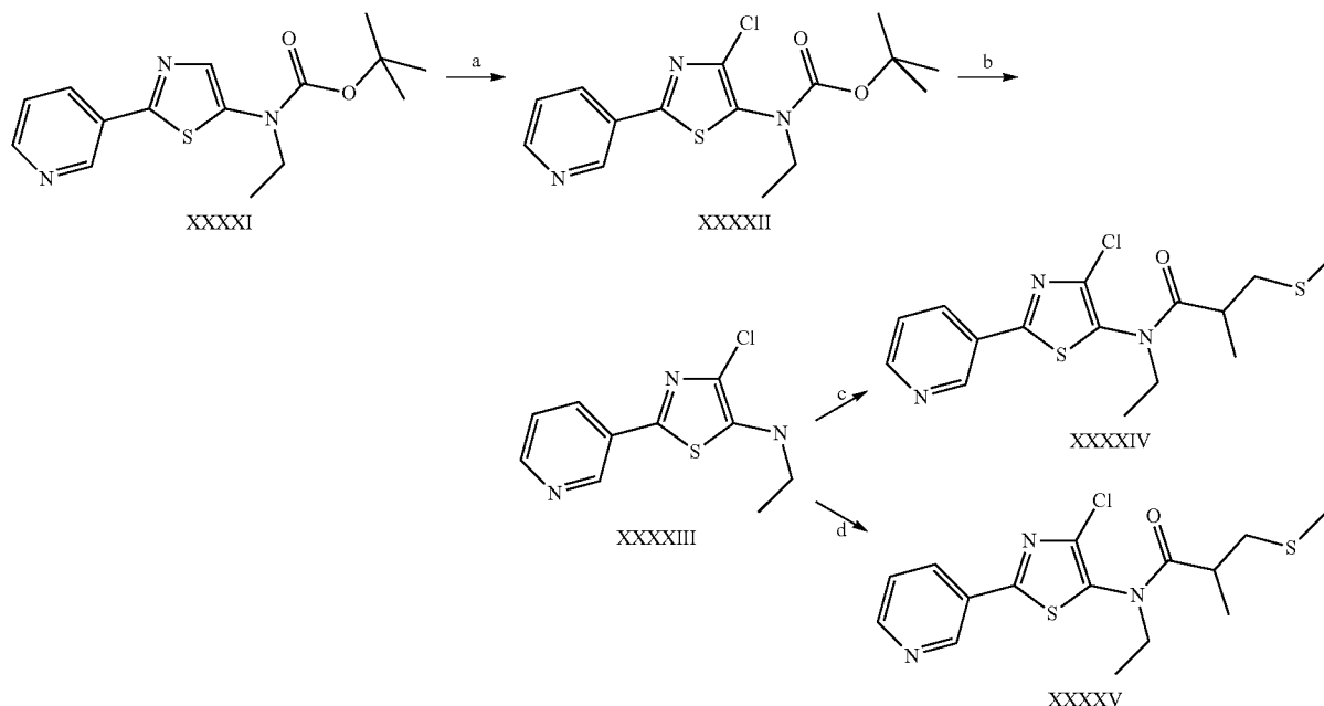
Scheme XXI
