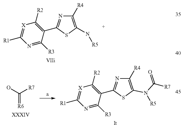
Scheme XVI
