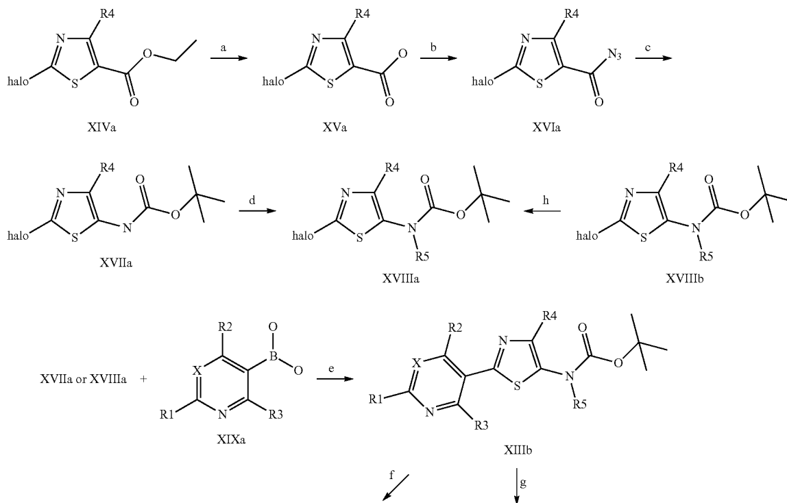
Scheme III
