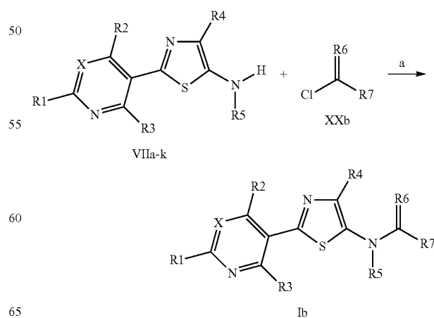
Scheme V
