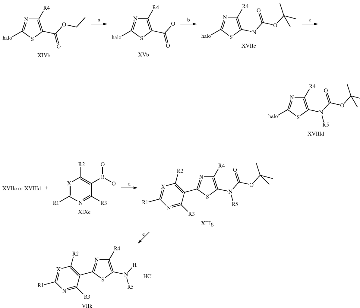
Scheme XVIII
