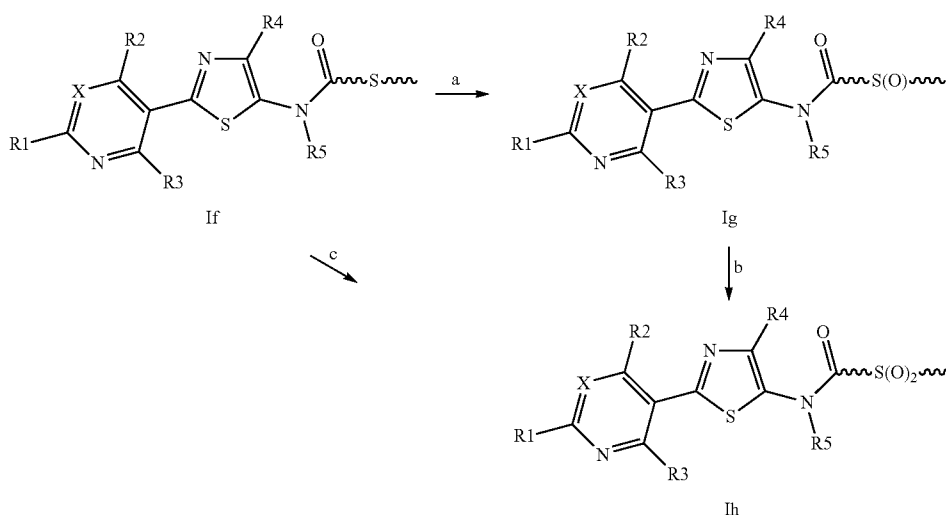
Scheme VII
