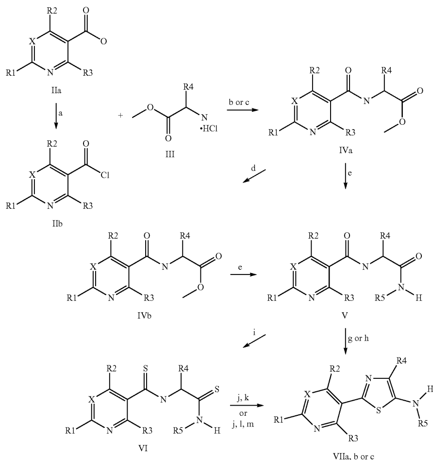
Scheme I
