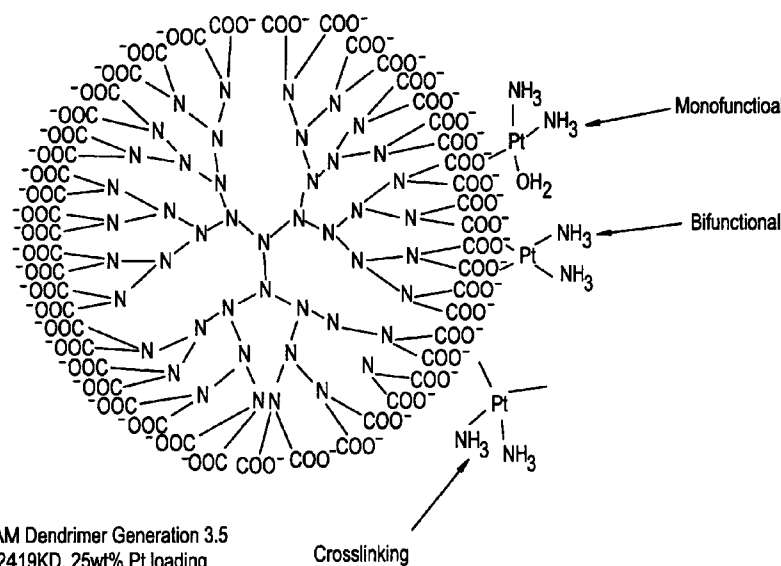
Possible variations in platinum binding to dendrimer
