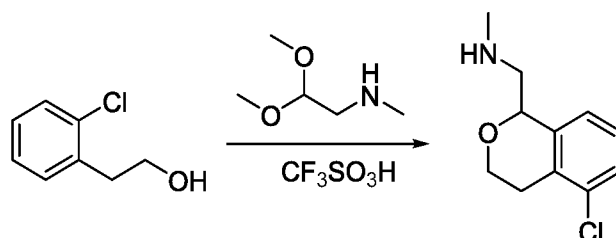
(a). 1-(5-chloroisochroman-1-yl)-N-methylmethanamine
