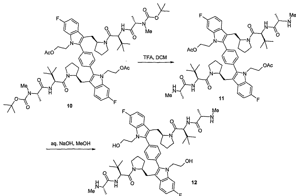
Scheme V
