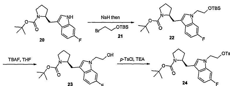
Scheme VIII
