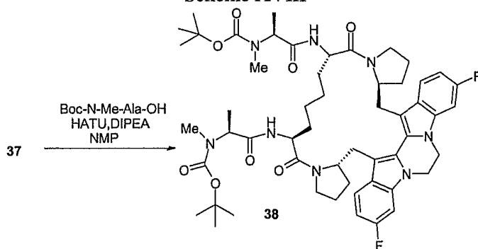
Scheme XVIII
