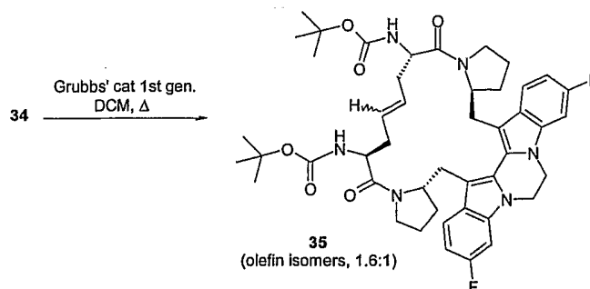
Scheme XV
