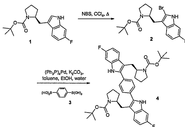
Scheme I
