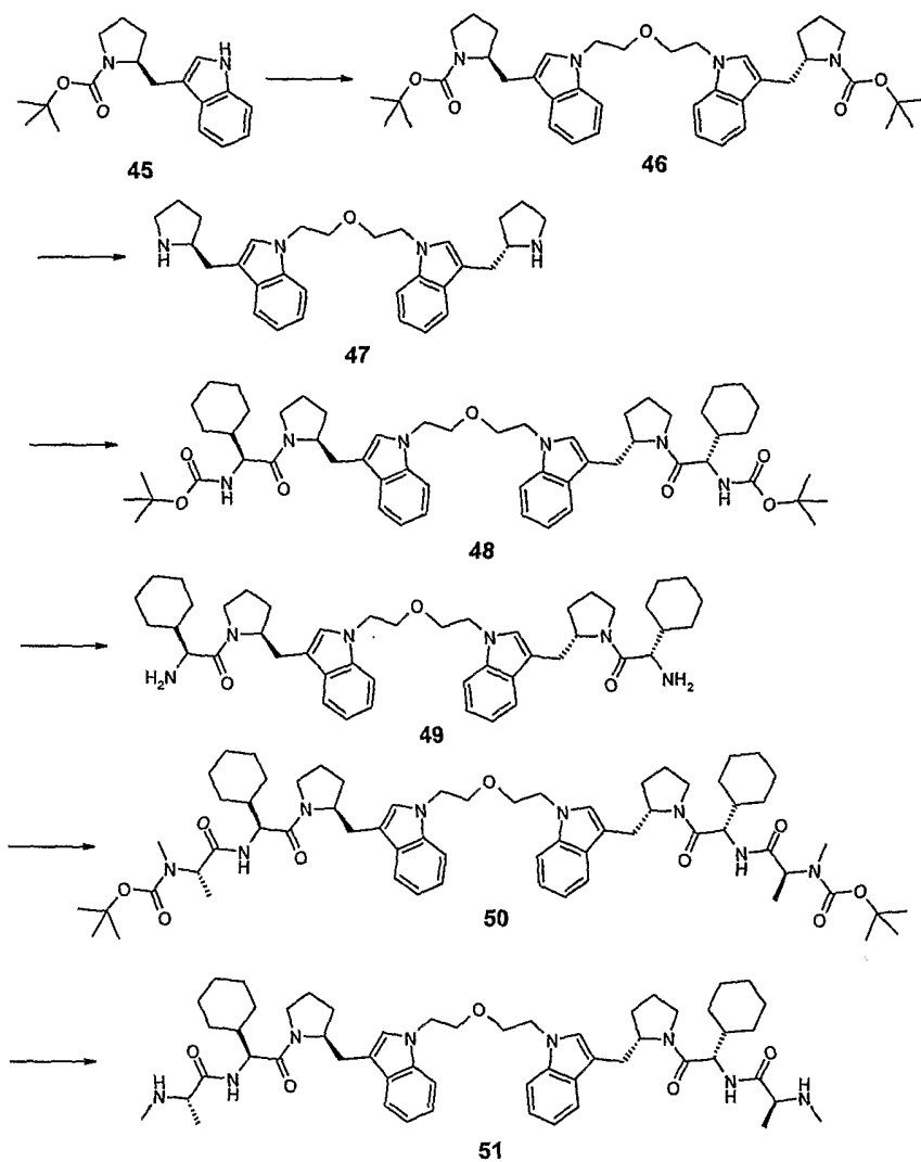
Scheme XXI
