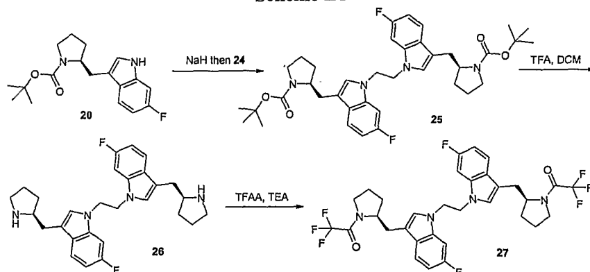
Scheme IX
