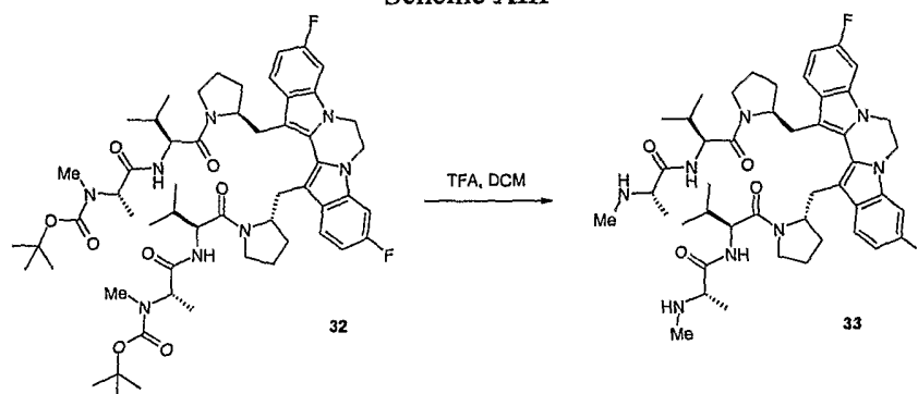
Scheme XIII
