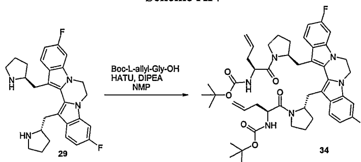
Bis-(Boc-Allylglycine)-containing Species (34)
