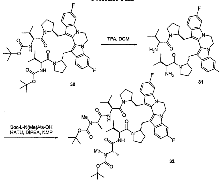
Scheme XII
