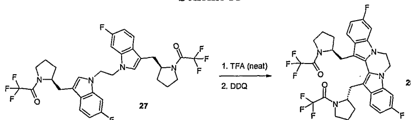
Scheme X
