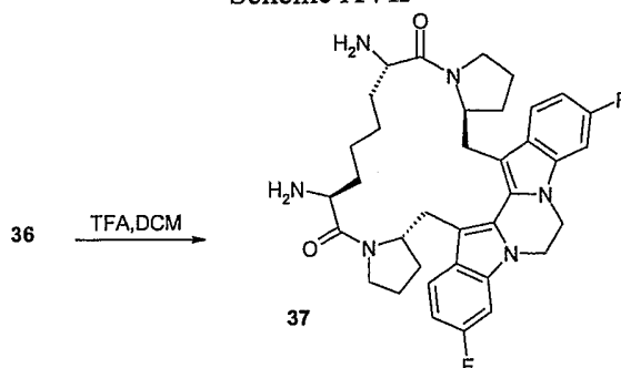
Scheme XVII
