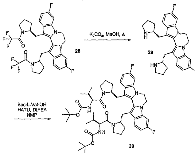
Scheme XI
