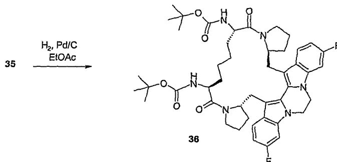
Scheme XVI
