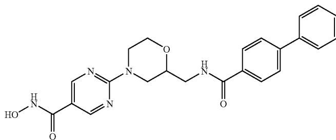
Co. No. 8; Ex. [B8]; mp. 290° C.
