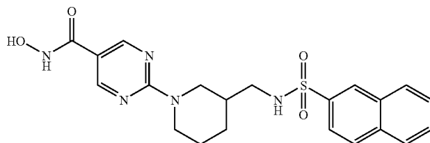
Co. No. 10; Ex. [B10]; mp. 210° C.
