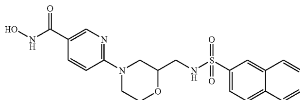
Co. No. 7; Ex. [B7]; mp. 157° C.
