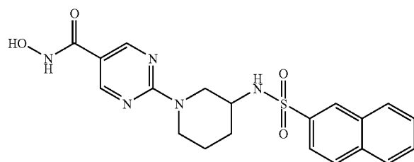
Co. No. 14; Ex. [B10], mp. 150° C.
