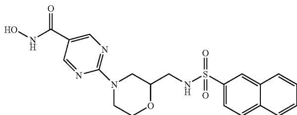
Co. No. 6; Ex. [B6]; mp 179° C.
