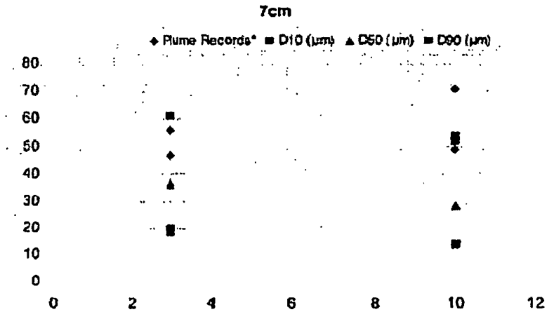
Figure 13: Exhaust Results Dv10, Dv50, Dv90 vs. Distance to Exhaust at 7 cm Device to Laser Beam
