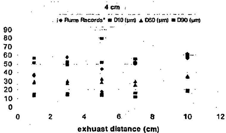
Figure 12: Exhaust Results Dv10, Dv50, Dv90 vs. Distance to Exhaust at 4 cm Device to Laser Beam
