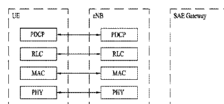
(b) User-plane protocol stack
