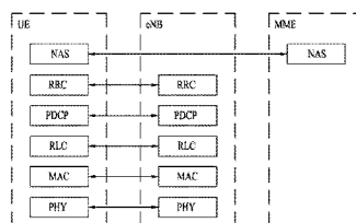
(a) Control-plane protocol stack
