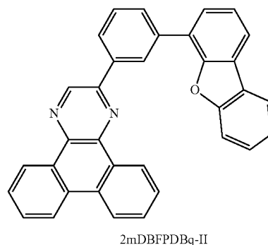
[Chemical Formula 104]
