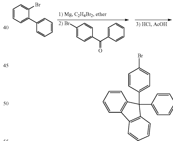
[Chemical Formula 110]
