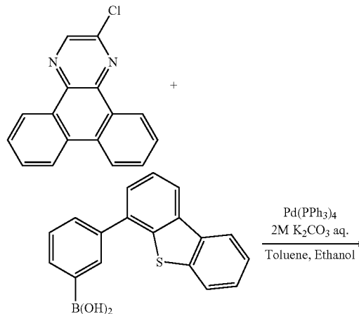
[Chemical Formula 77]
