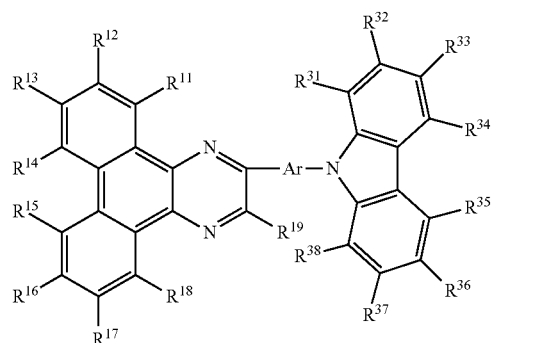
[Chemical Formula 8]
