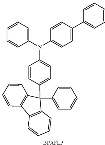
[Chemical Formula 109]
