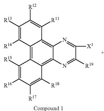
[Chemical Formula 72]
