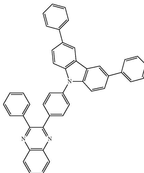
Cz1PQ-III
