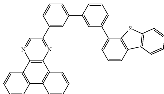
[Chemical Formula 84]
