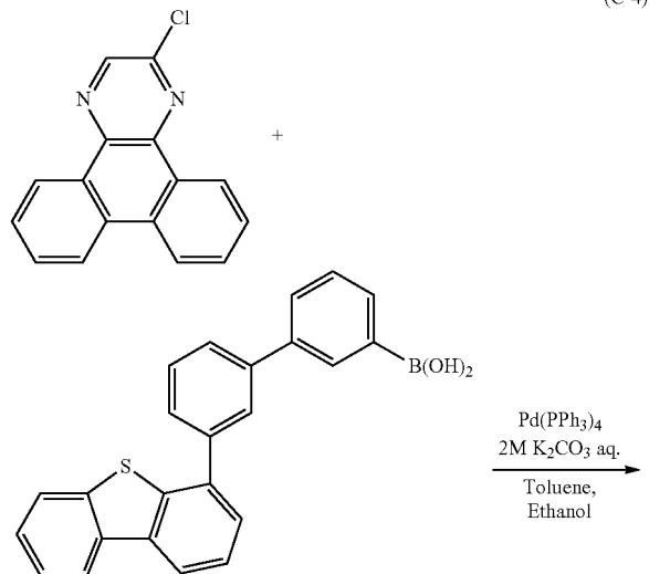
[Chemical Formula 85]
