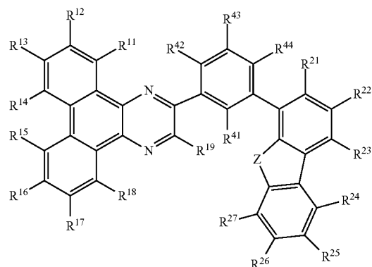
(G3-1)
