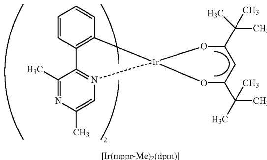
[Chemical Formula 112]
