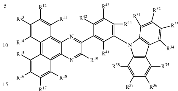
[Chemical Formula 10]
