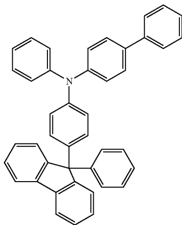
BPAFLP
