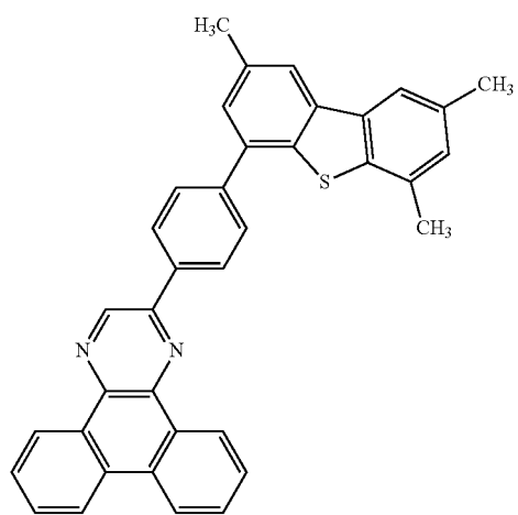
[Chemical Formula 17]
