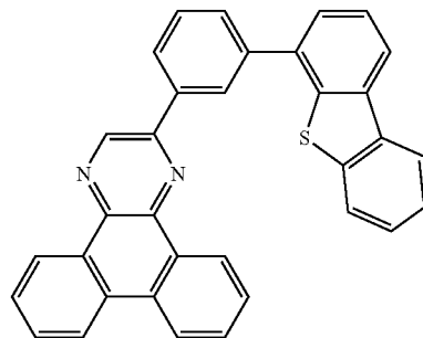
[Chemical Formula 76]
