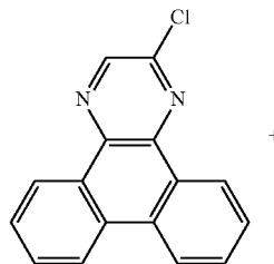
[Chemical Formula 83]
