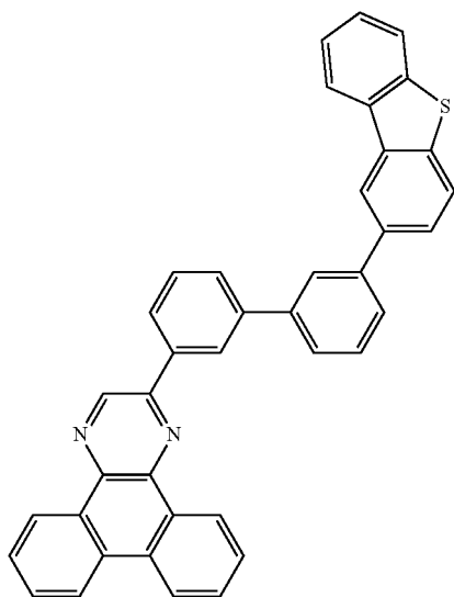
[Chemical Formula 55]
