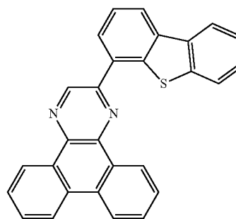
[Chemical Formula 82]
