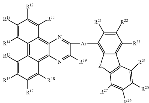
(G2-1)
