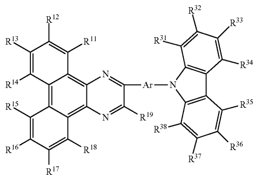
[Chemical Formula 3]
