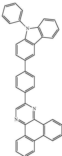
[Chemical Formula 96]
