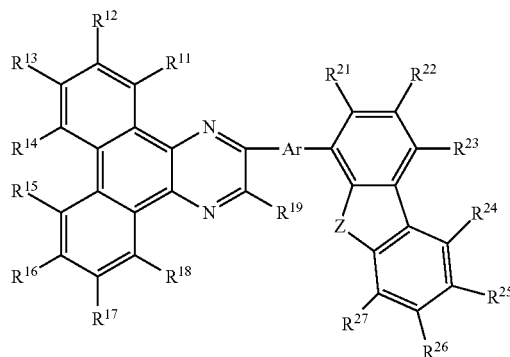
[Chemical Formula 7]
