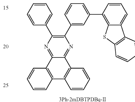
[Chemical Formula 103]
