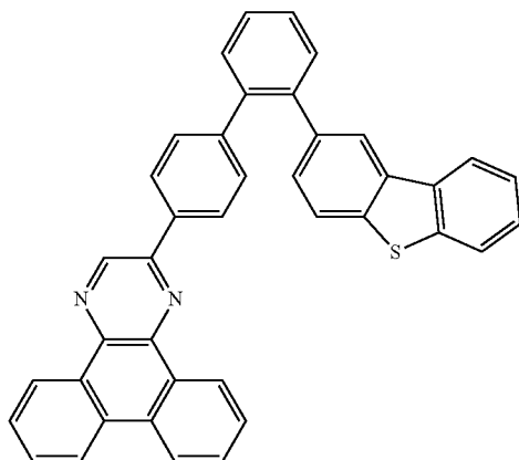
[Chemical Formula 55]
