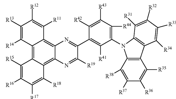
(G3-2)
