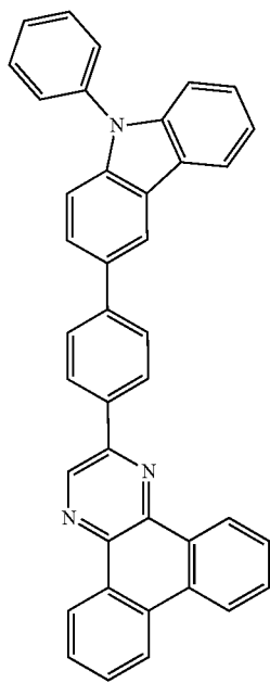
PCPDBq
