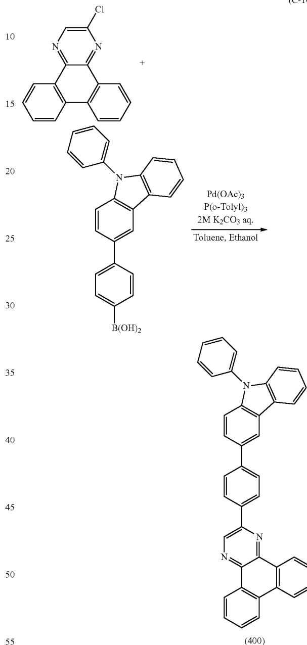
[Chemical Formula 97]
