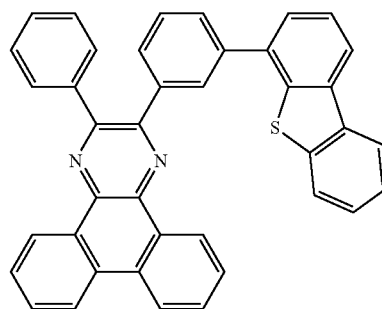
[Chemical Formula 88]
