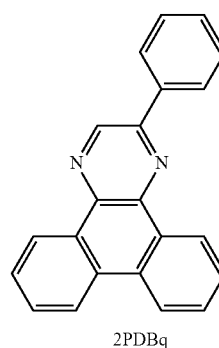
[Chemical Formula 108]
