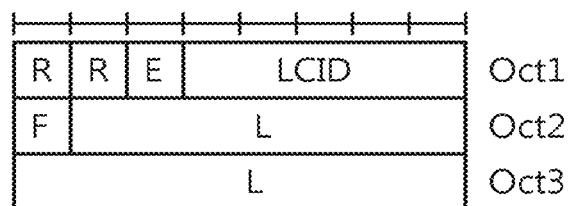
(B) R/R/E/LCID/F/L sub-header with 15-bit L field
