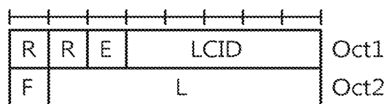
(A) R/R/E/LCID/F/L sub-header with 7-bit L field
