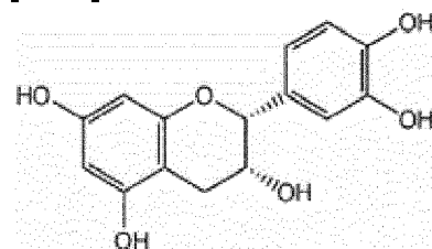
(-)-Epicatechin (2R,3R)
