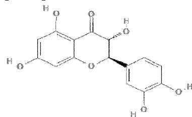
Taxifolin
