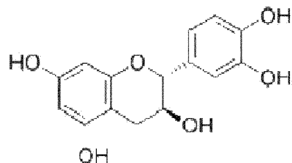
Catechin
