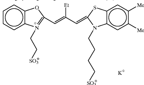
Sensitizing dye for green light-sensitive emulsion (14)
