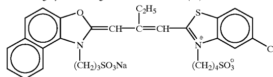
Sensitizing dye for red light-sensitive emulsion (17)
