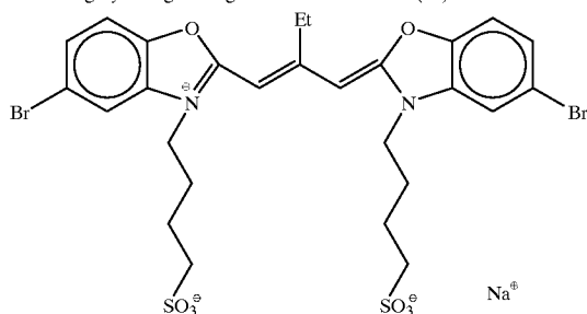
Sensitizing dye for green light-sensitive emulsion (14)
