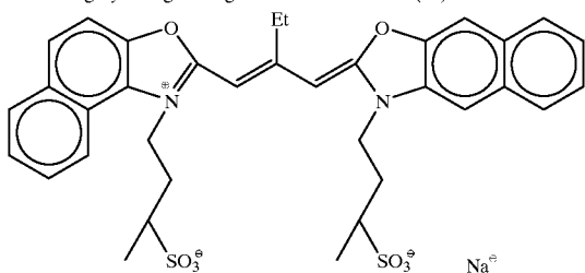
Sensitizing dye for green light-sensitive emulsion (14)
