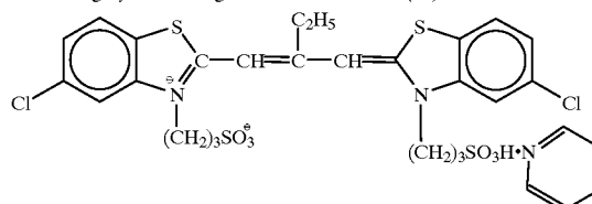
Sensitizing dye for red light-sensitive emulsion (18)
