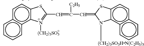
Sensitizing dye for red light-sensitive emulsion (18)
