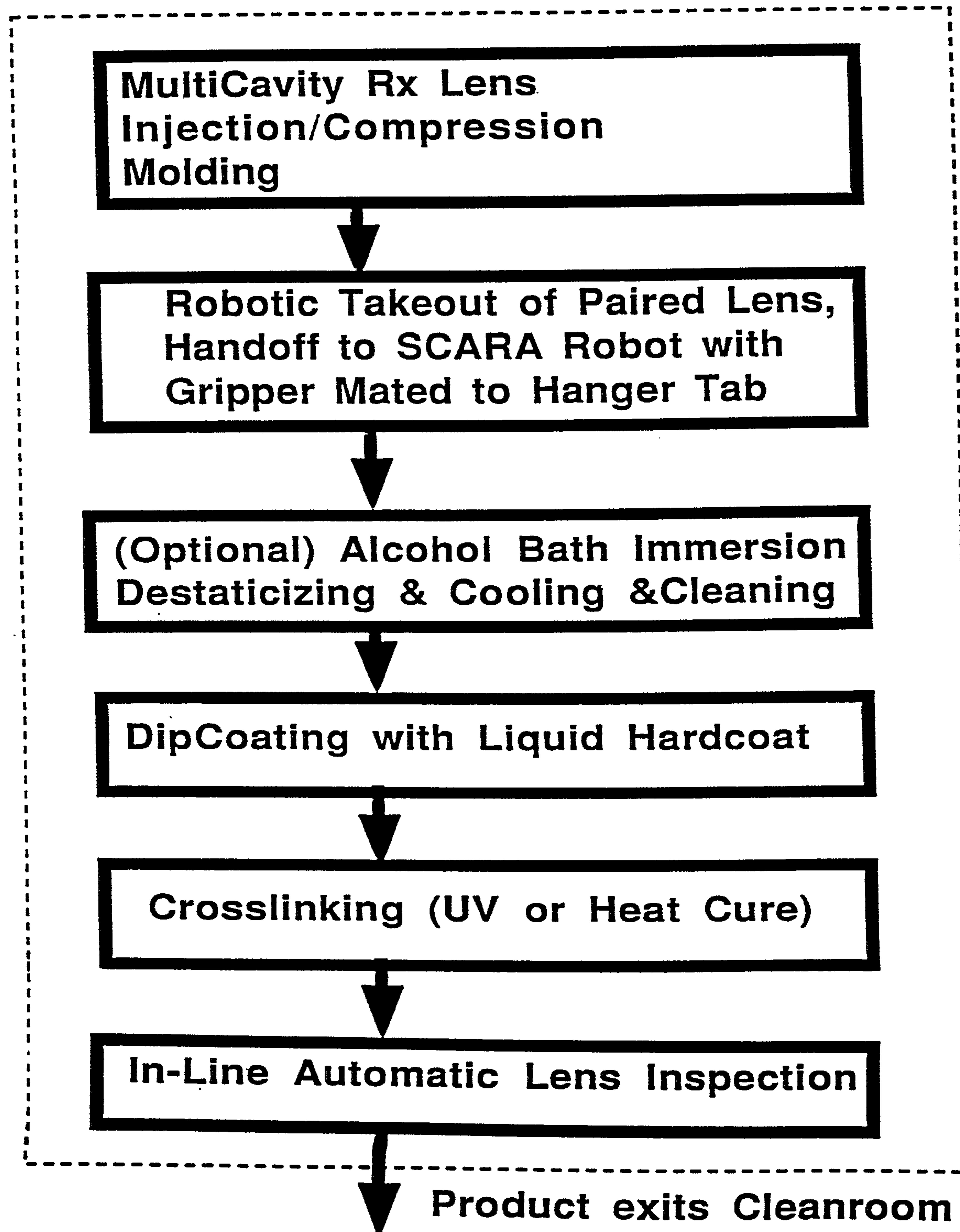
Figure 4C: In-Line Automated Inspection of "Mold and Dipcoat" ("Continuous Process")
