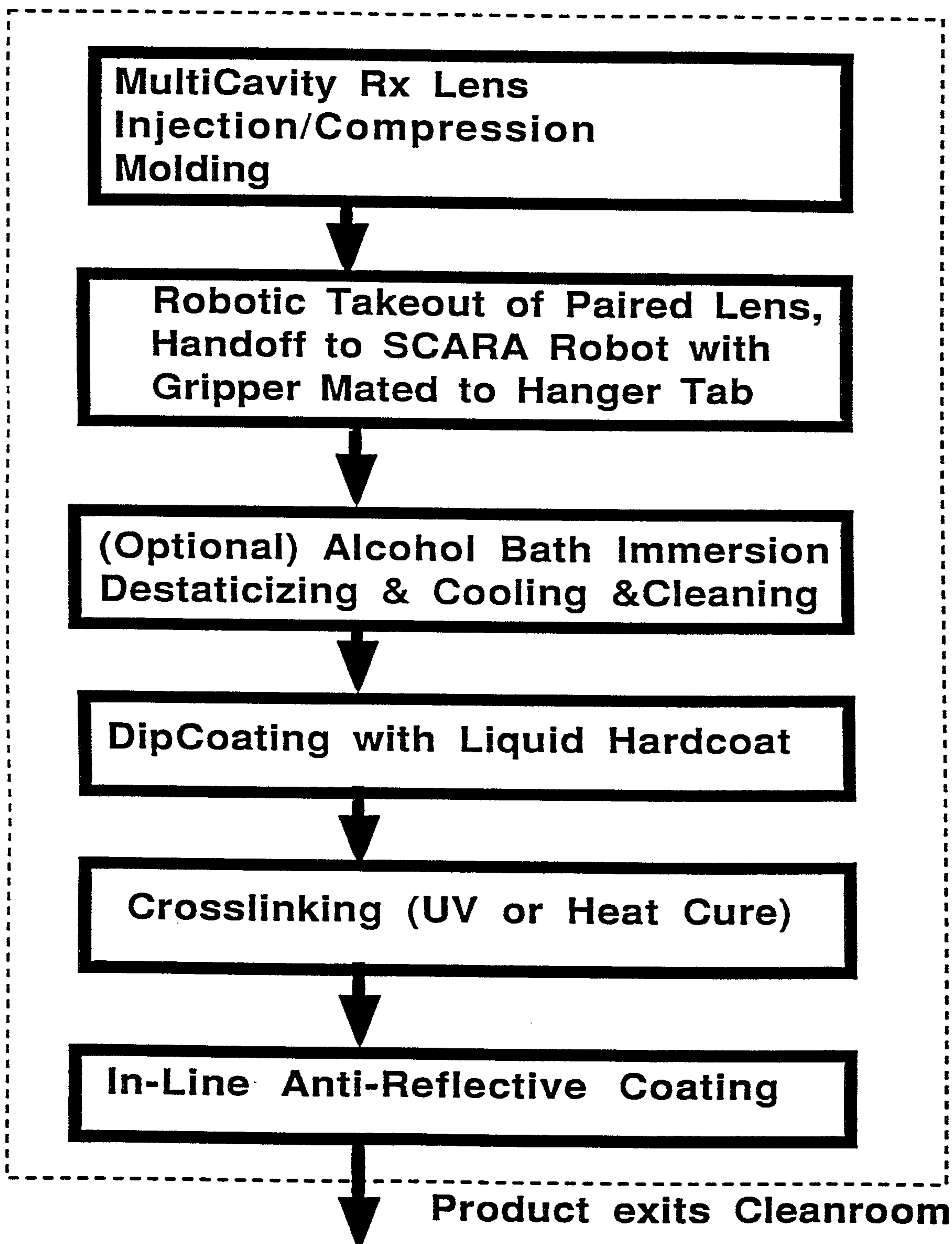
Figure 4D: In-Line Automated AR Vacuum Coat of "Mold and Dipcoat" ("Continuous Process")
