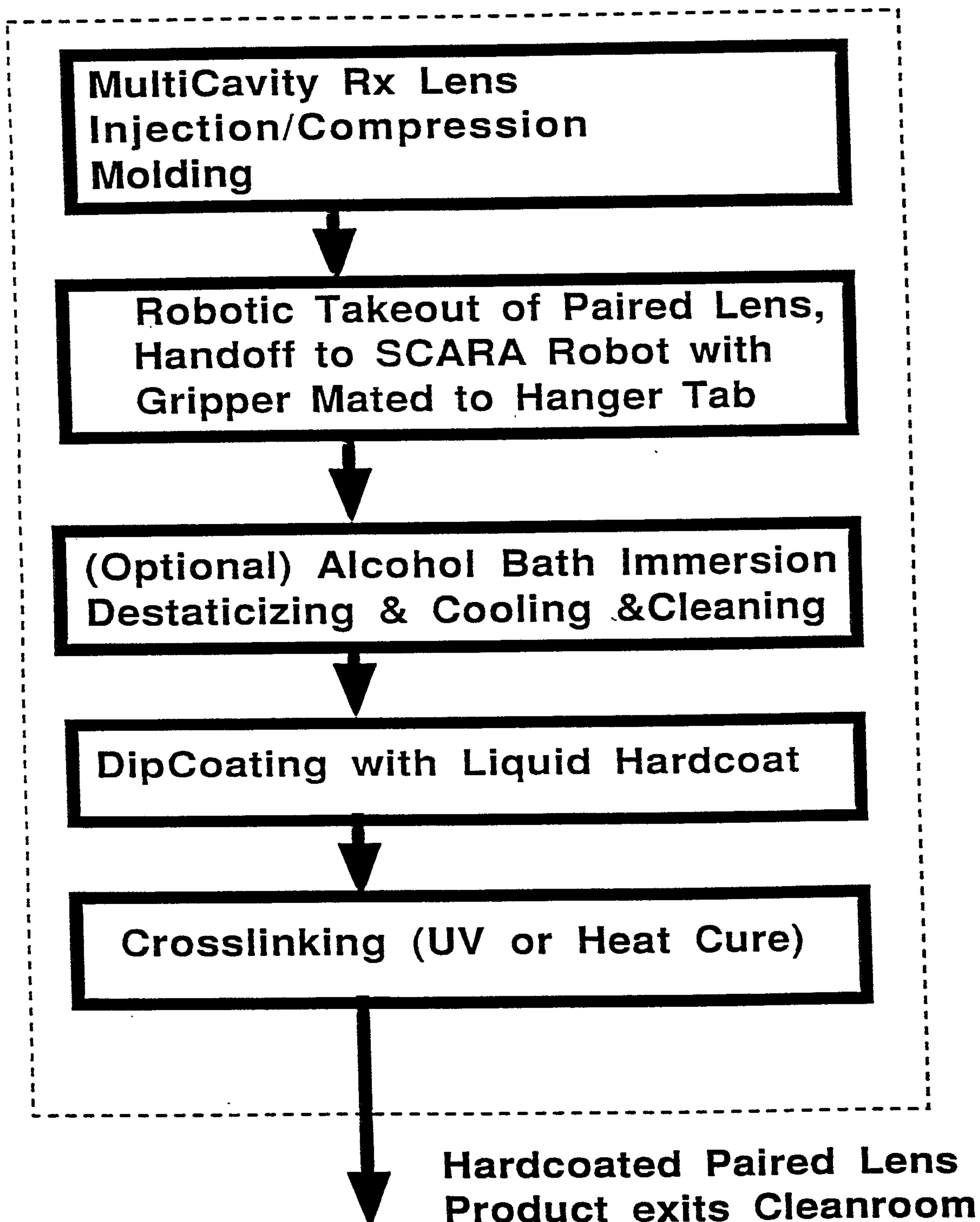
Figure 4B: Automated "Mold and Dipcoat" ("Continuous Process")
