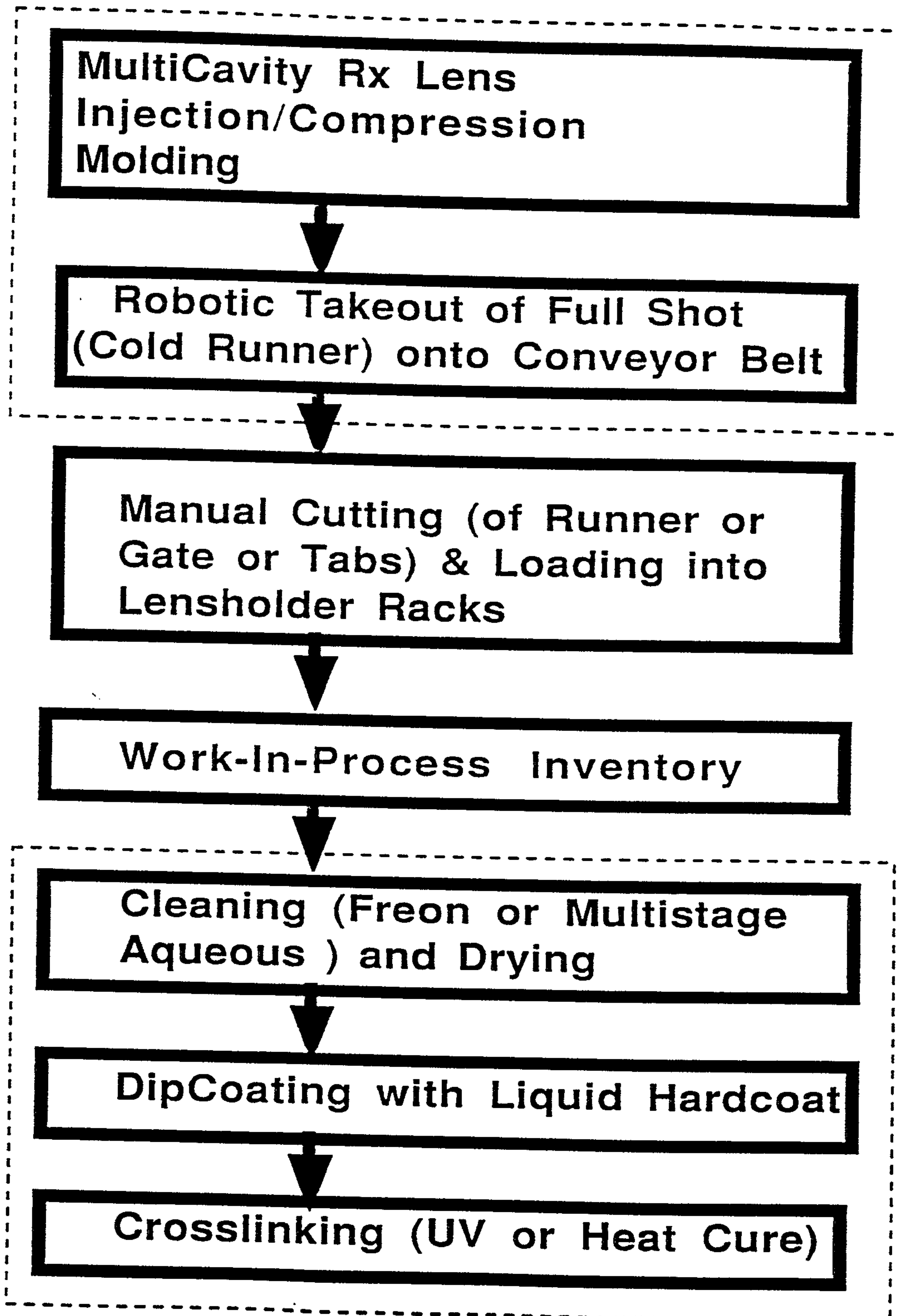
Figure 4A: Comparative Example ("Batch Process")
