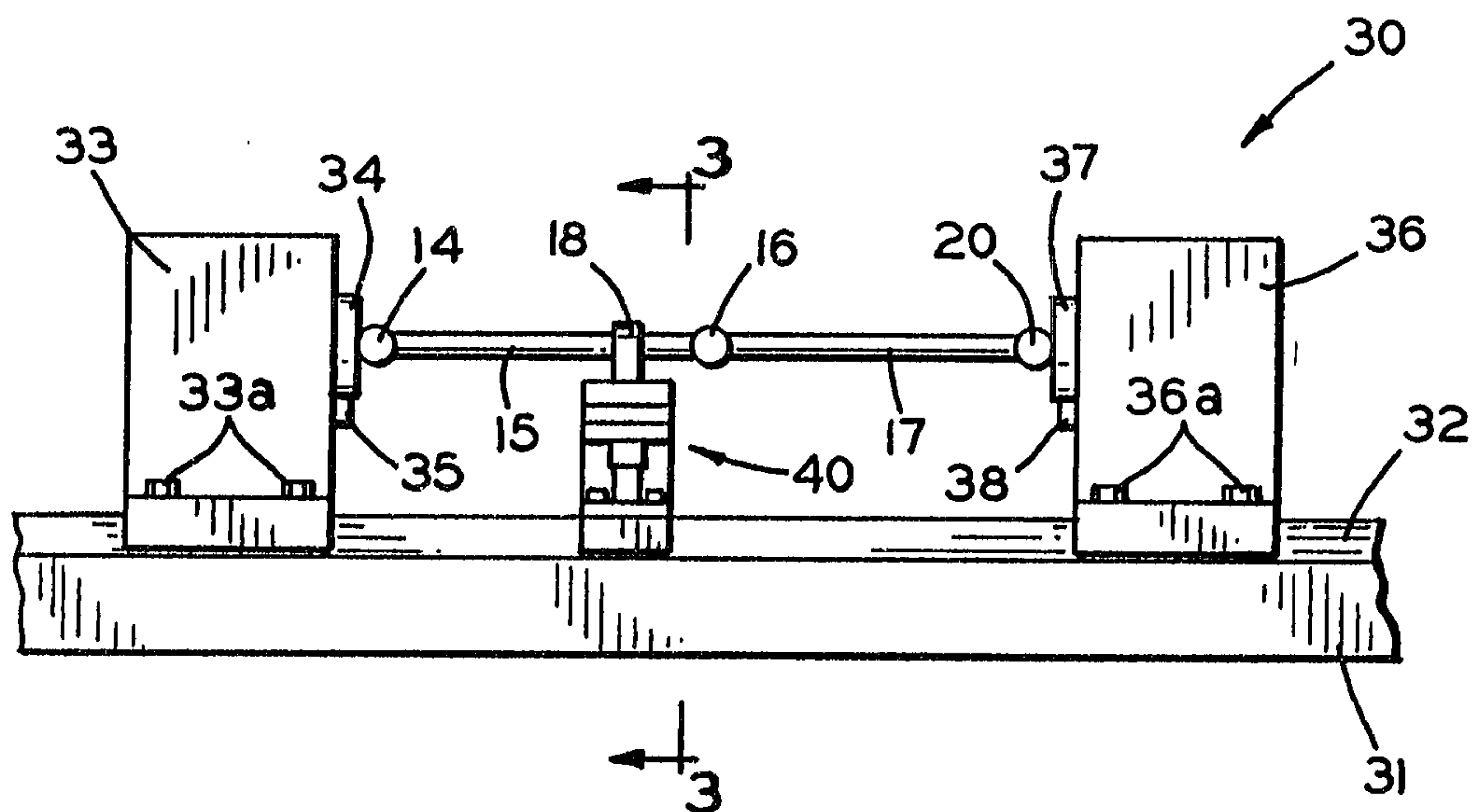
FIG. 2 (PRIOR ART)
