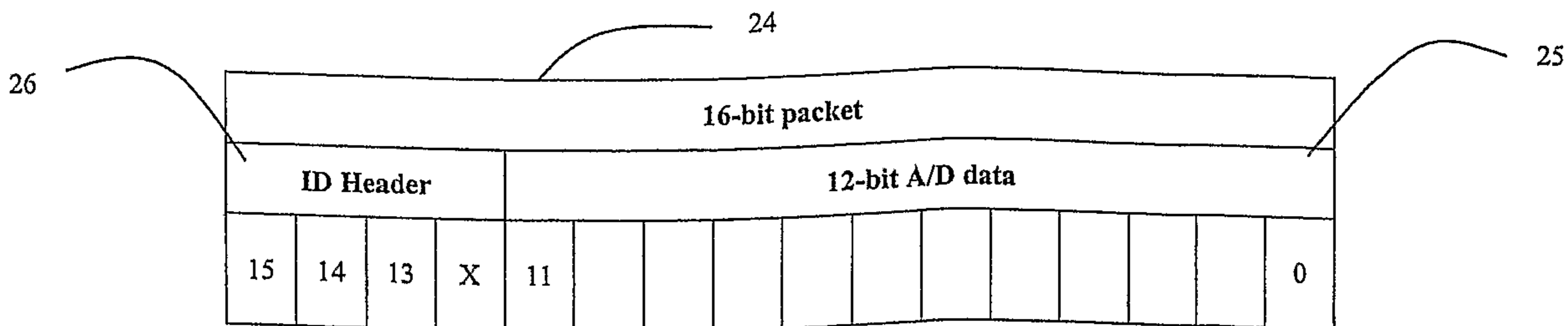
Figure 5a: Transmission Data Format
