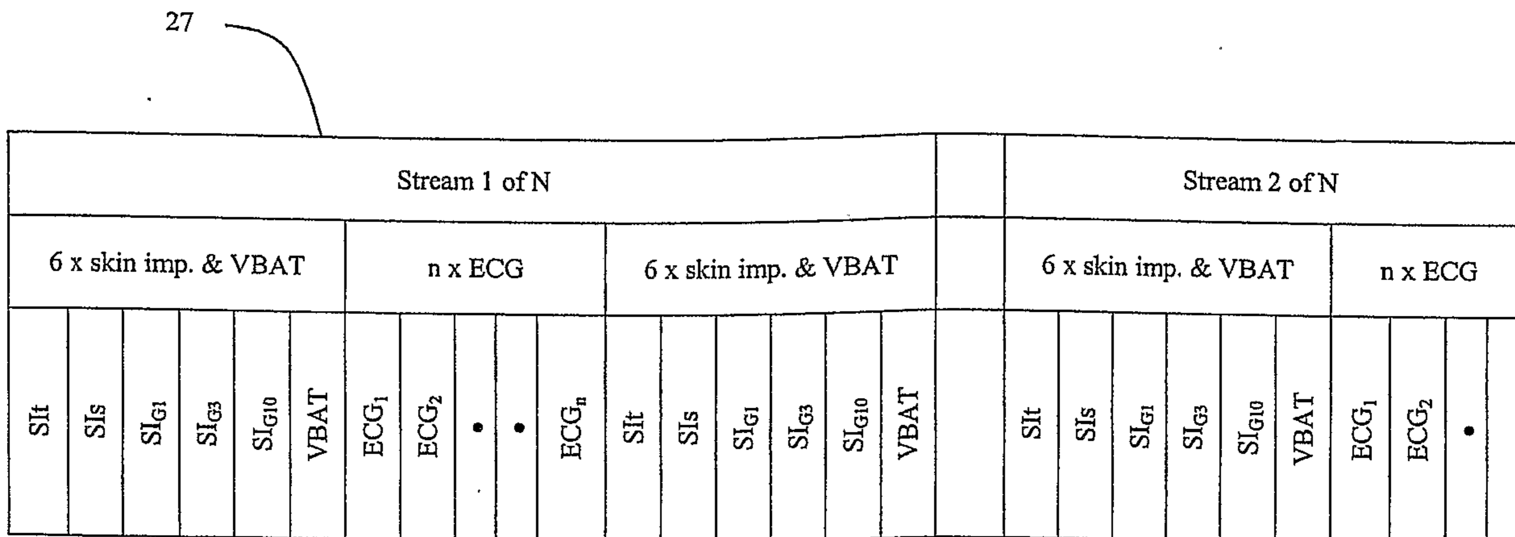
Figure 5c: Transmitter data sequence stream
