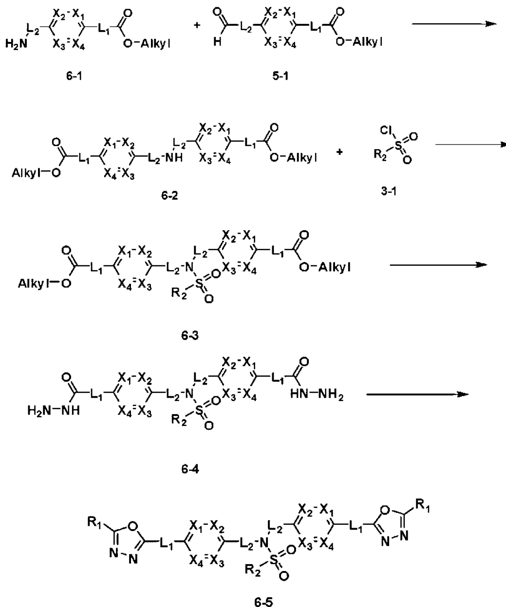
[Reaction Scheme 6]
