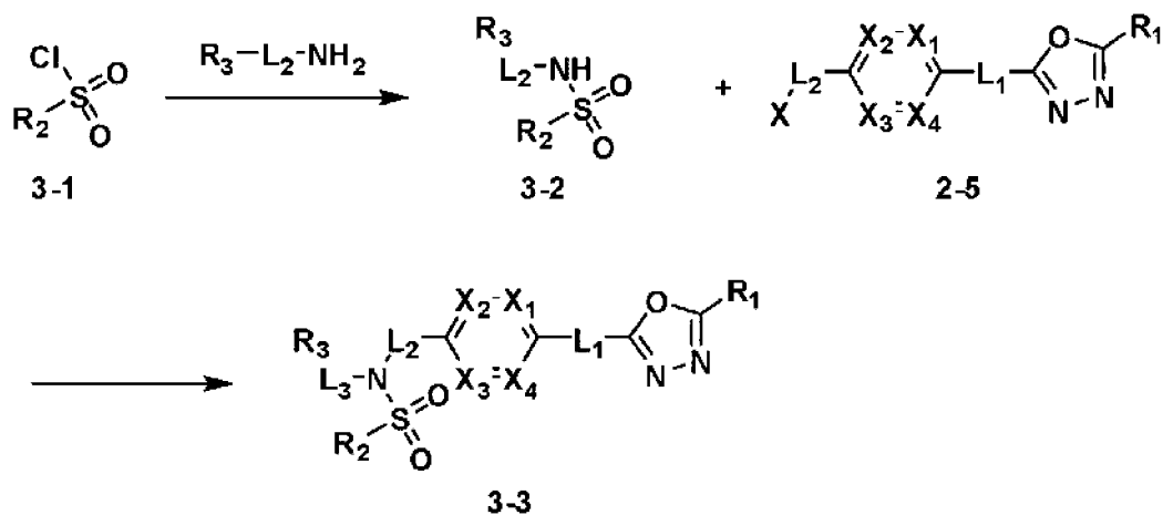
[Reaction Scheme 3]
