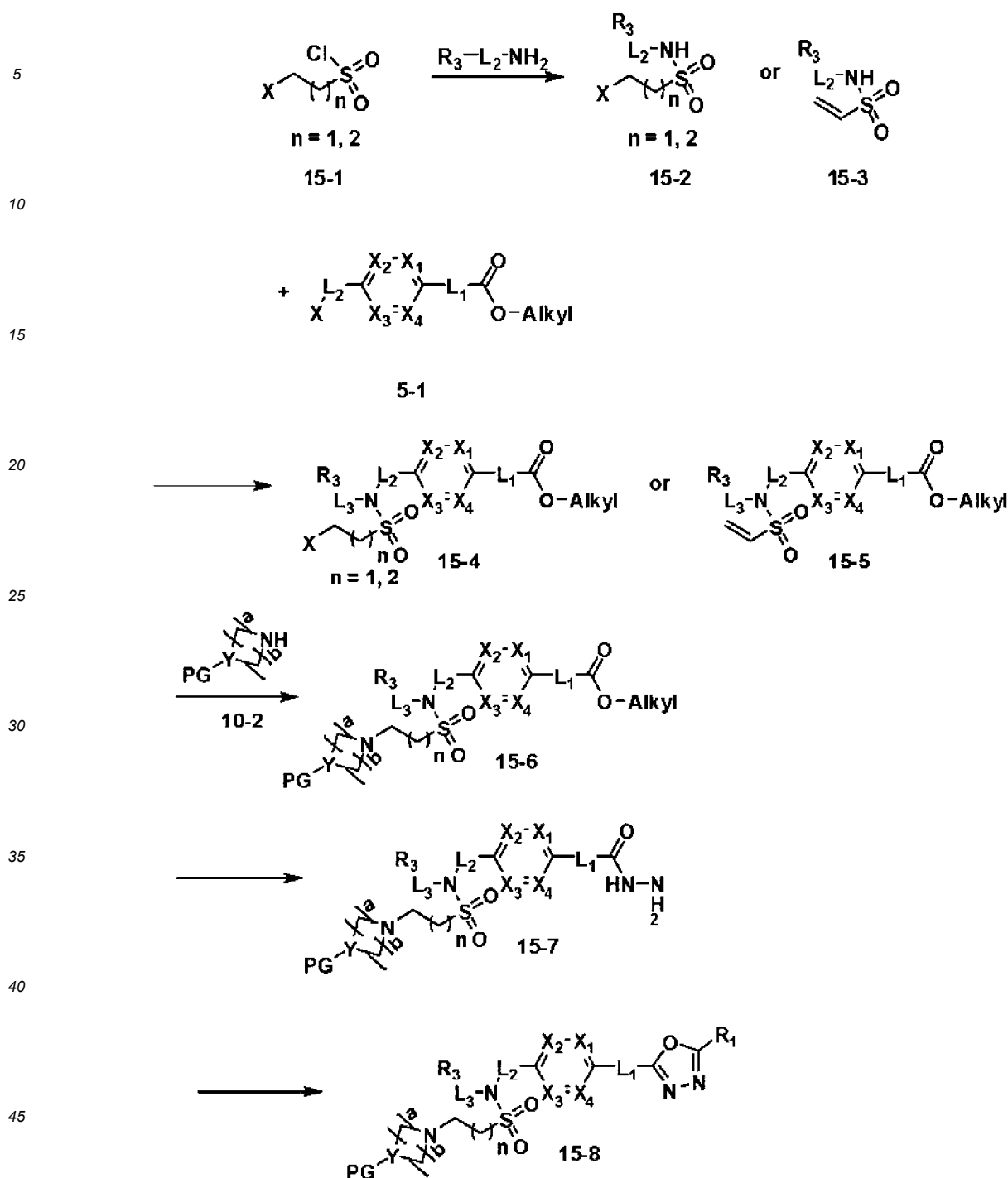
[Reaction Scheme 15]
