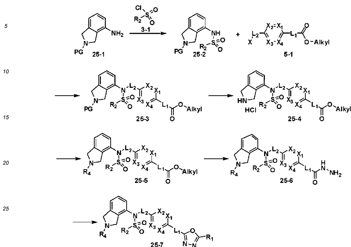
[Reaction Scheme 25]
