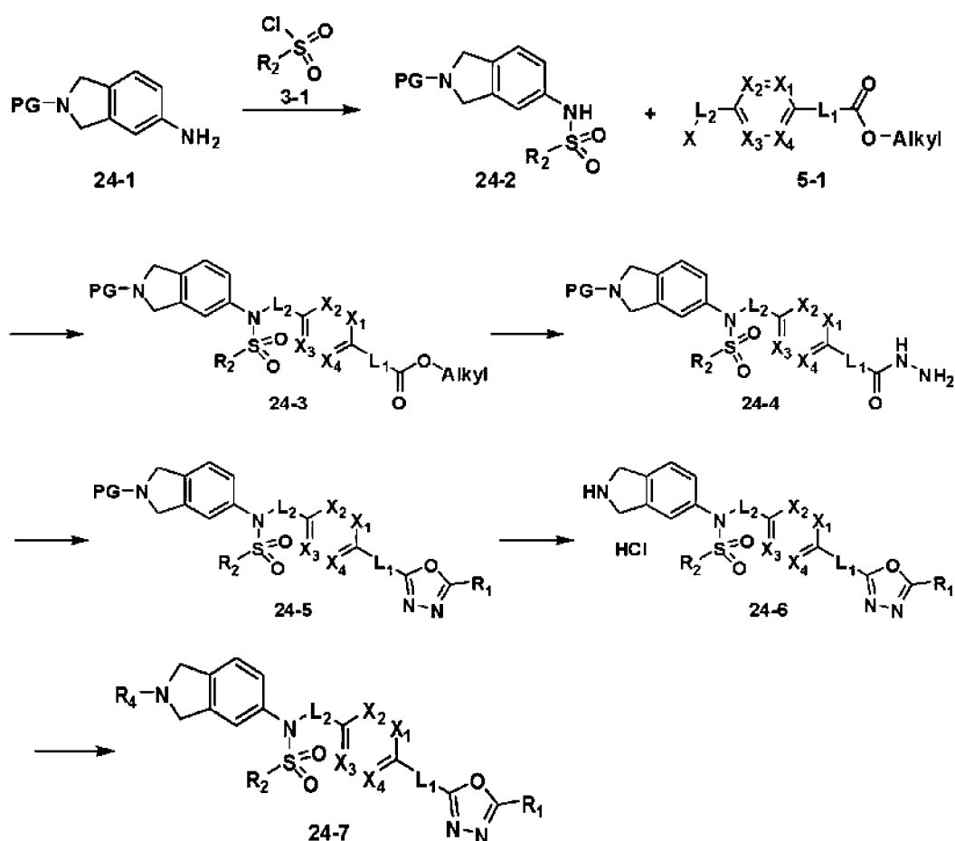
[Reaction Scheme 24]
