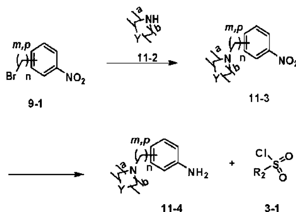
[Reaction Scheme 11]
