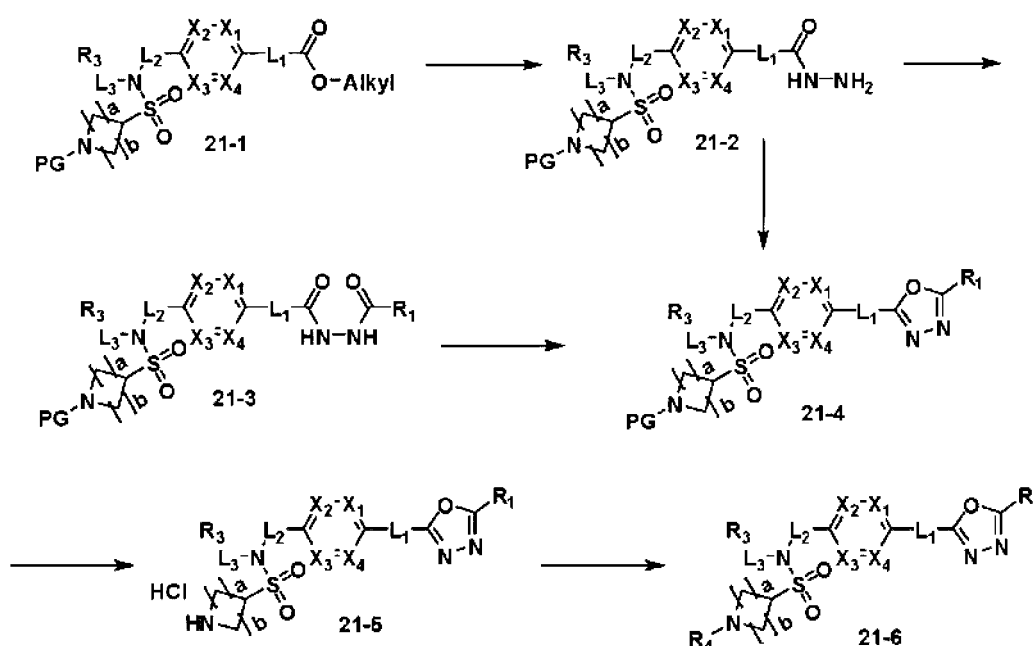
[Reaction Scheme 21]
