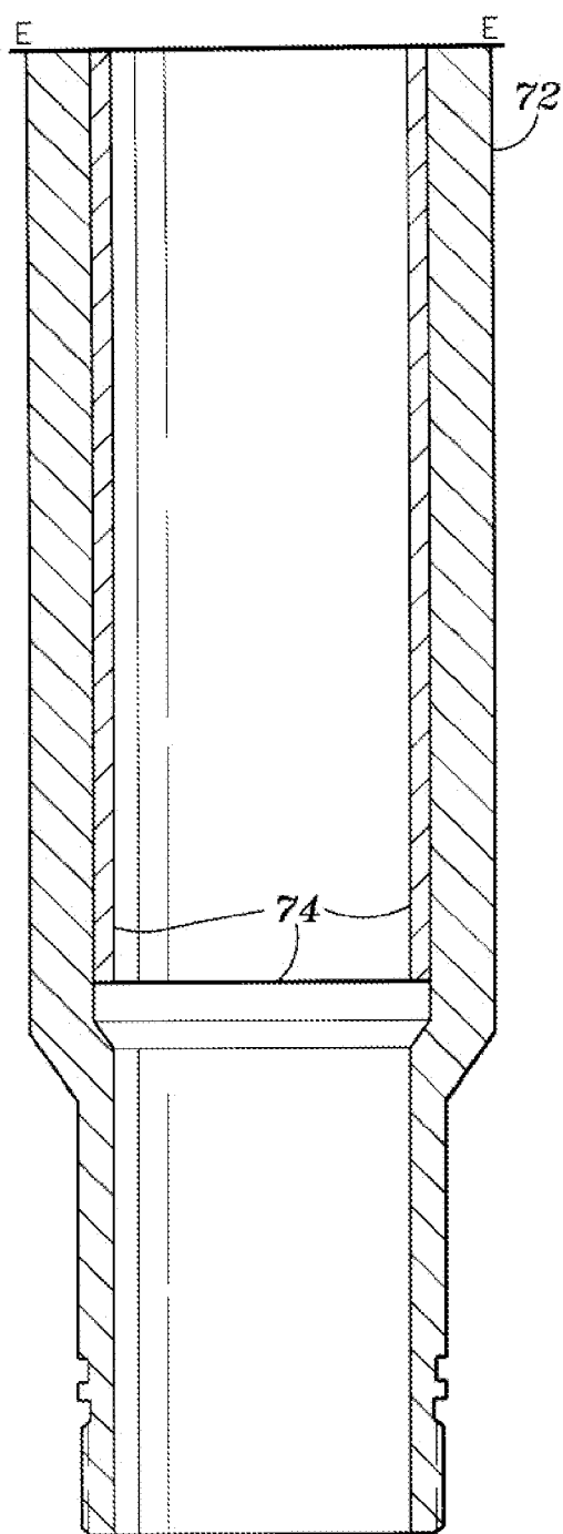
FIG. 2f DOWNHOLE OPEN
