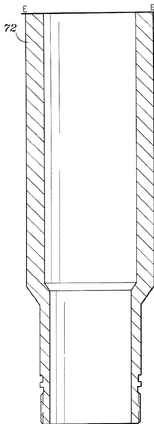
FIG. 3f DOWNHOLE CLOSED
