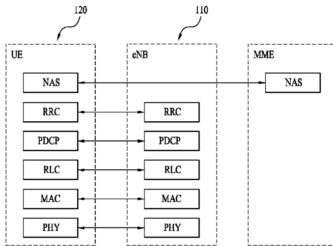
(a) Control-plane protocol stack
