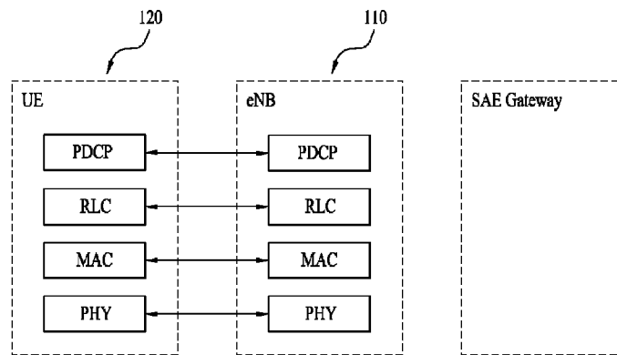
(b) User-plane protocol stack
