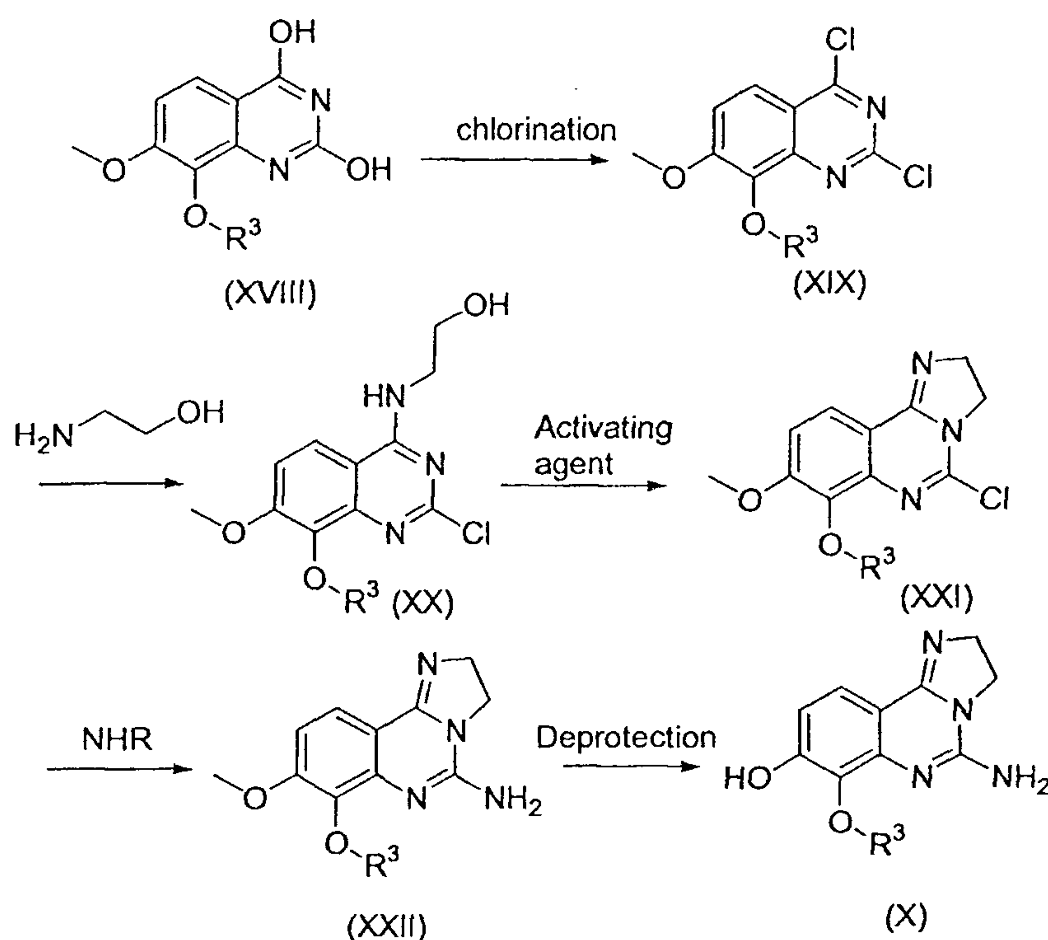
Reaction Scheme 5
