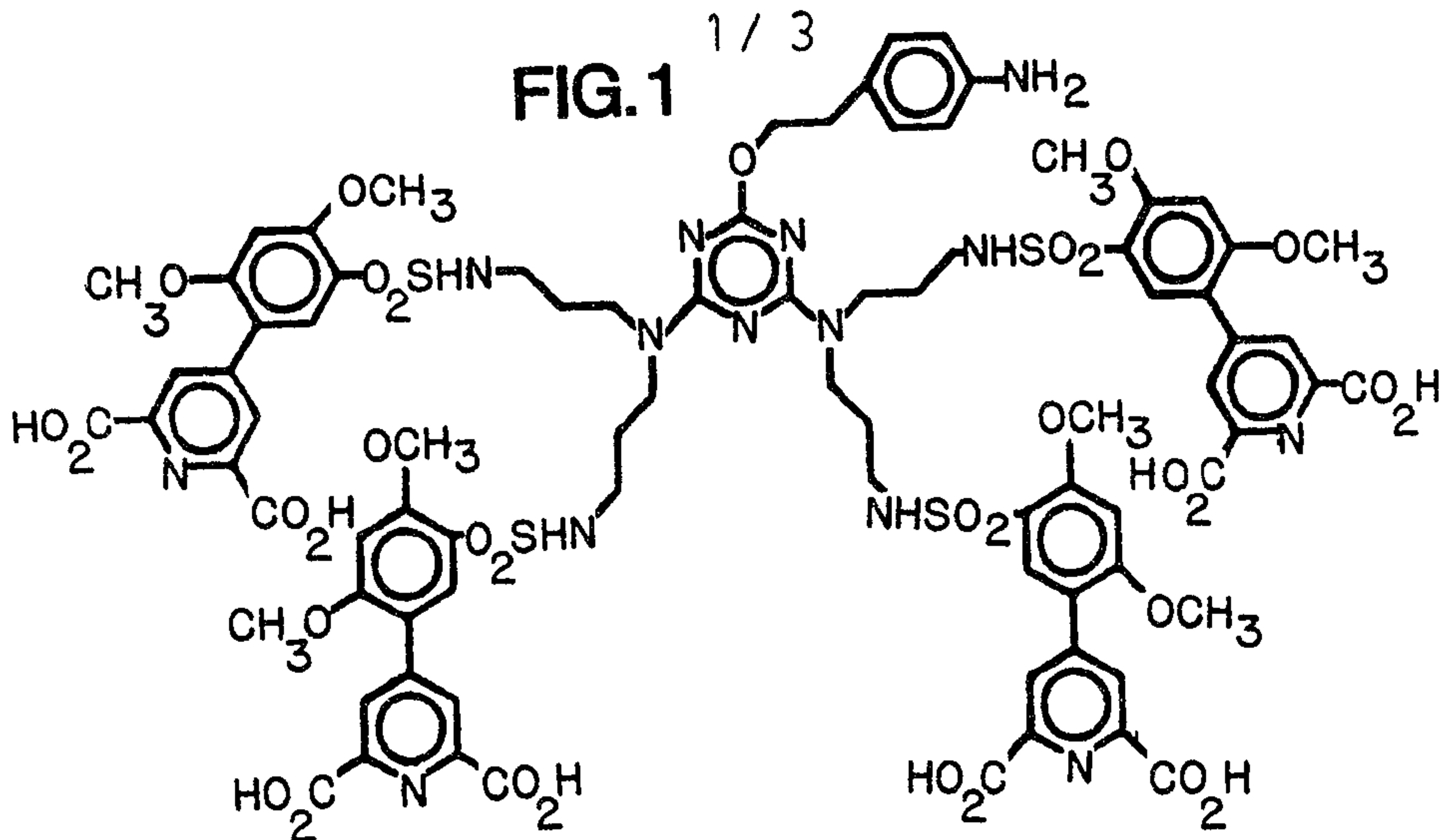
AMINO-TETRAKIS
