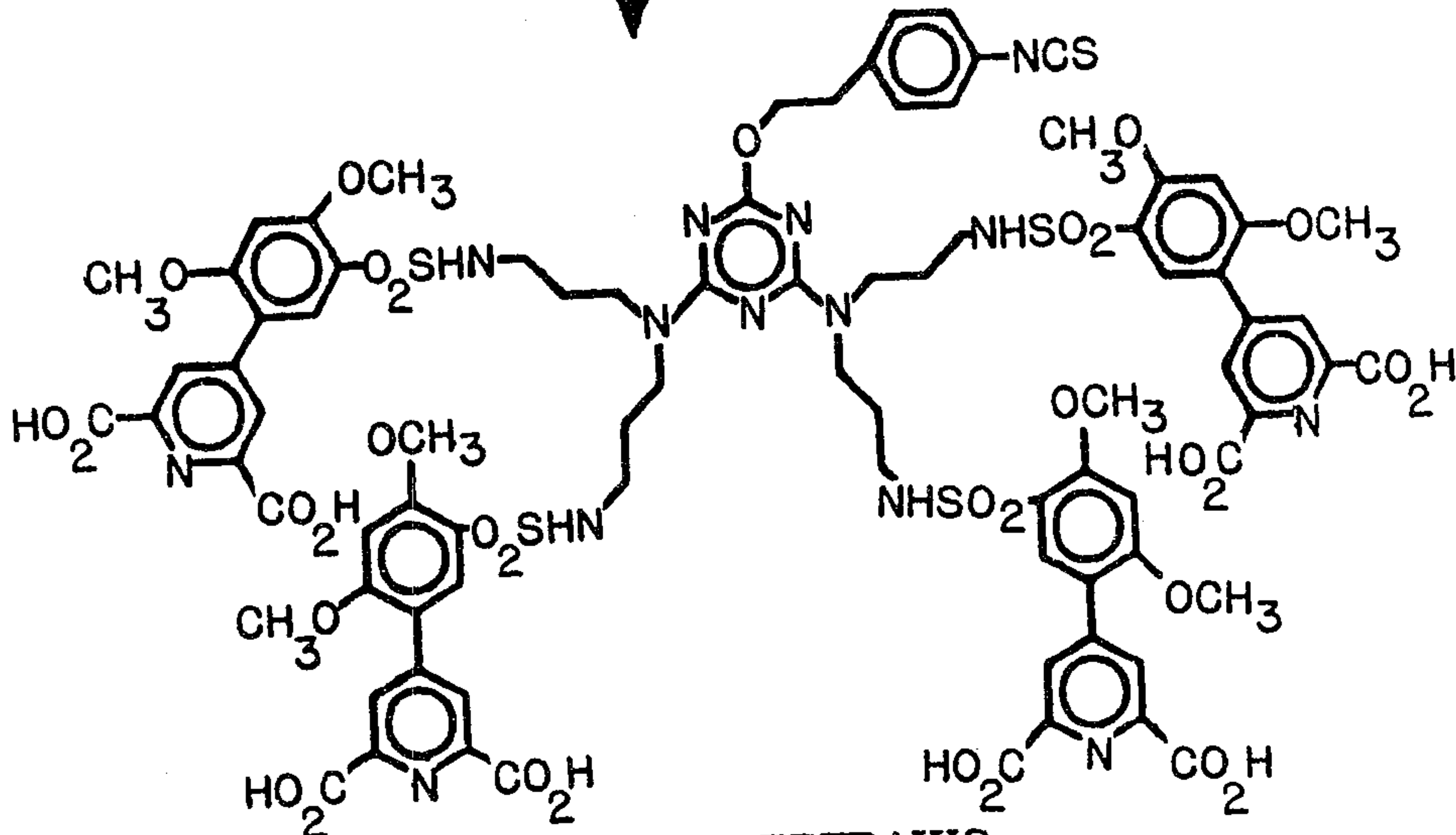
ISOTHIOCYANO-TETRAKIS (UNSTABLE)
