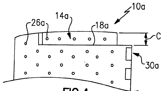
FIG. 4 Prior Art
