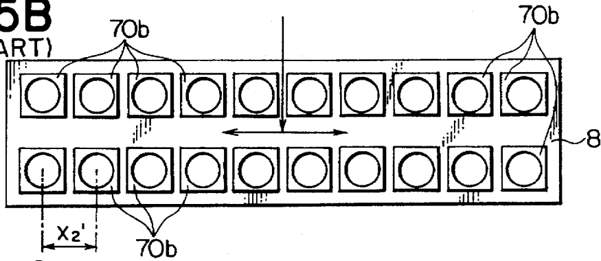
FIG. 5C (PRIOR ART)
