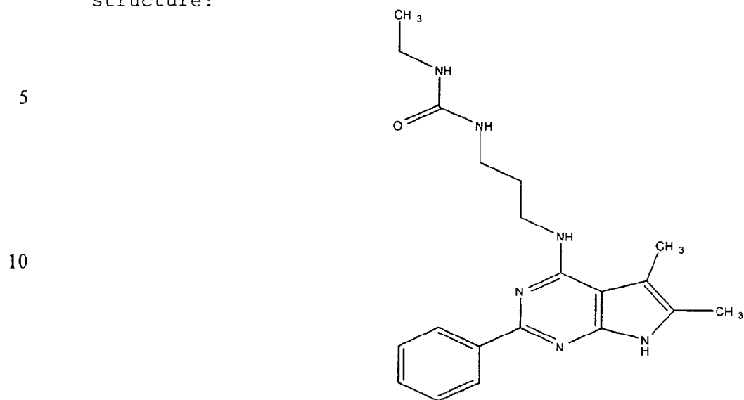
15 (Compound 1704)
