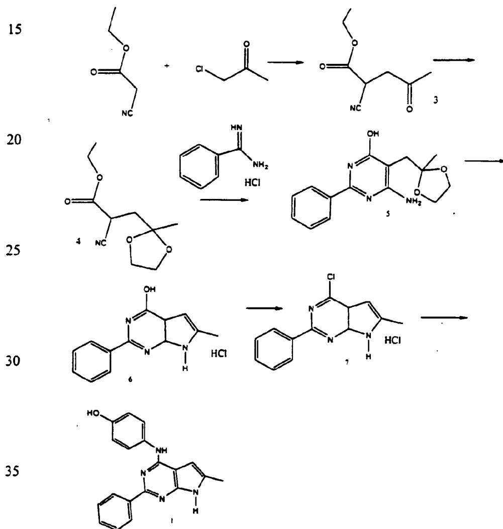
Scheme IV
