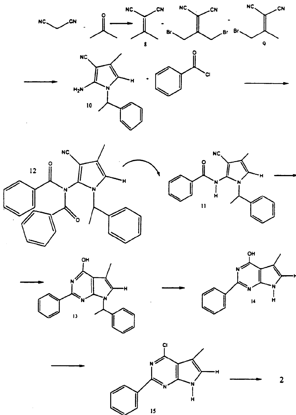
Scheme V
