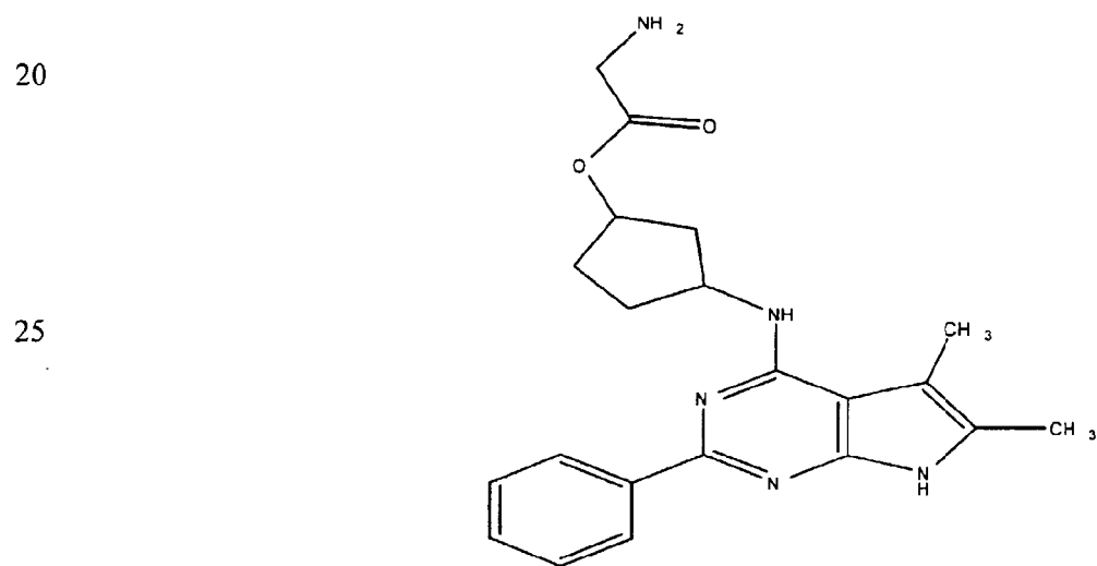
(Compound 1705)
