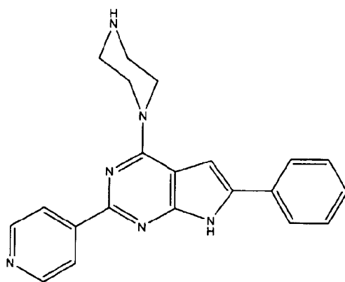
(Compound 1604)
