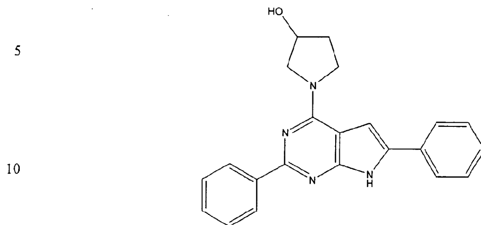
(Compound 1703)
