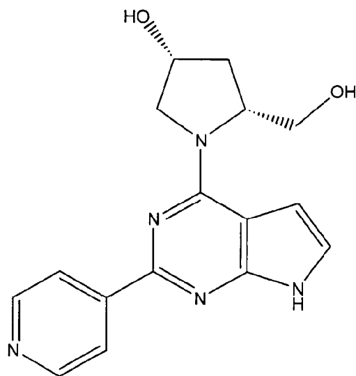
(Compound 1605)
