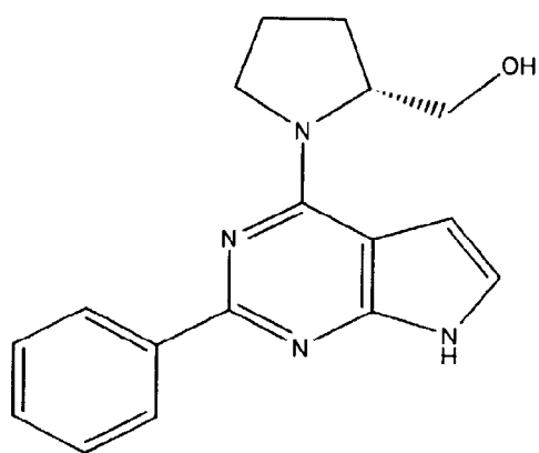
(Compound 1603)
