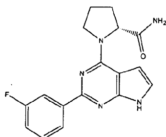
(Compound 1600)
