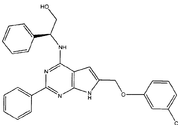
(Compound 1714)
