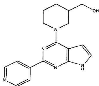
10 (Compound 1607)
