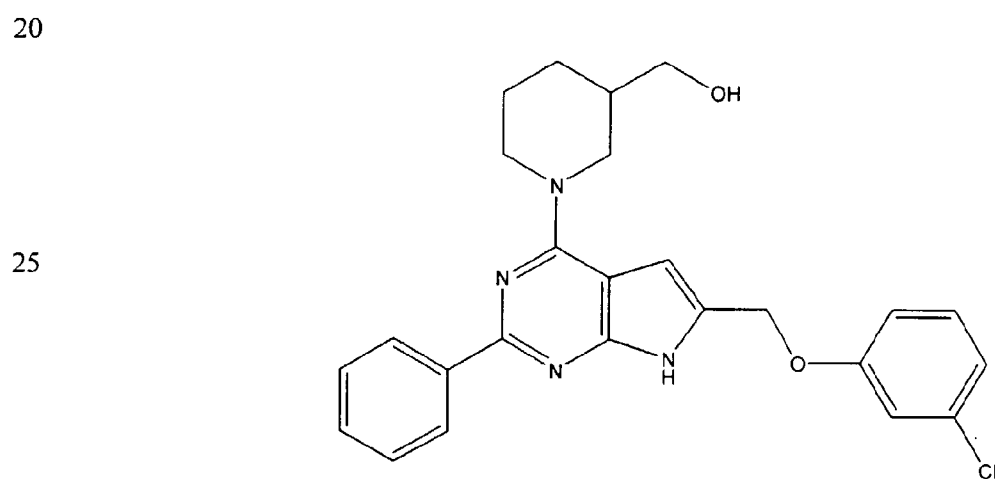
(Compound 1718)
