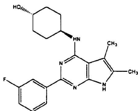
(Compound 706)
