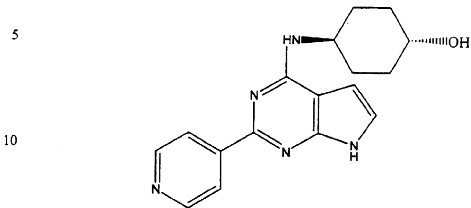
15 (Compound 1321)
