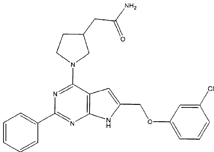
(Compound 1717)
