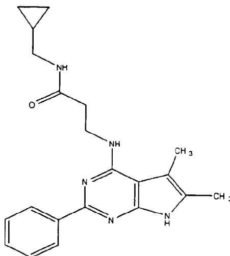
(Compound 1202)
