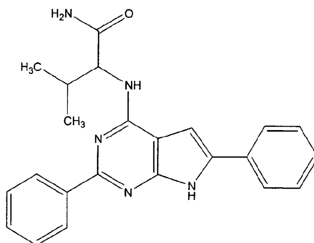
(Compound 1709)
