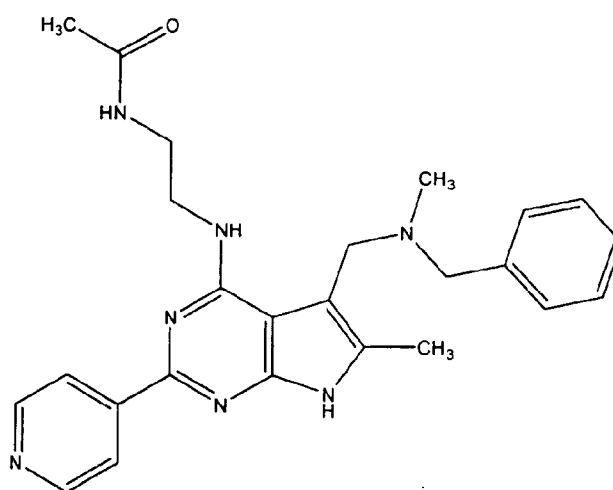
(Compound 1608)
