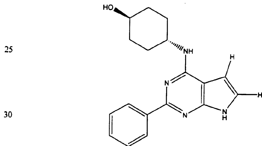
35 (Compound 1318-b)
