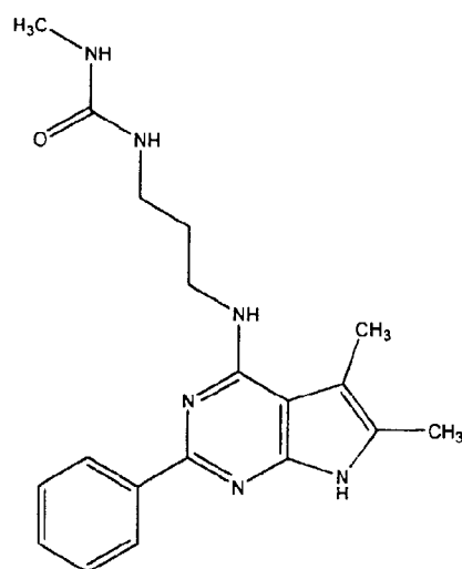
(Compound 1310)
