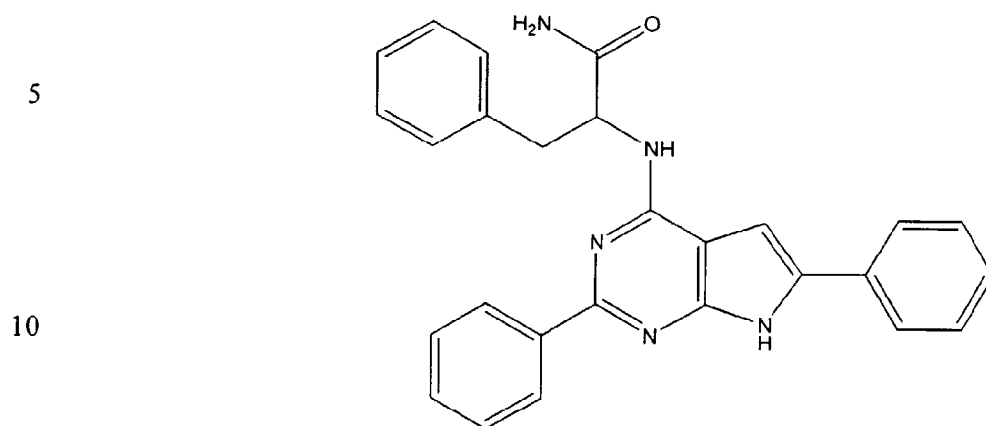
(Compound 1710)
