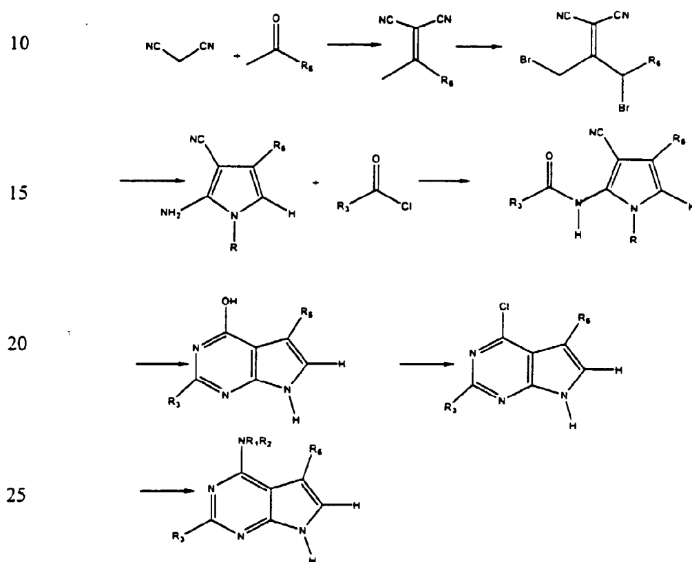
Scheme III
