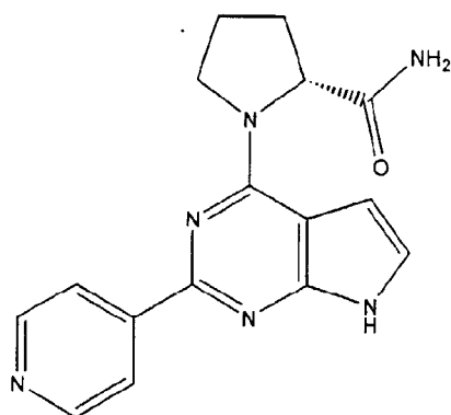
(Compound 1602) 30
