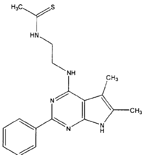
(Compound 1702)
