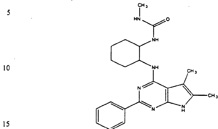
(Compound 1500)
