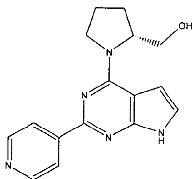
(Compound 1601) 15
