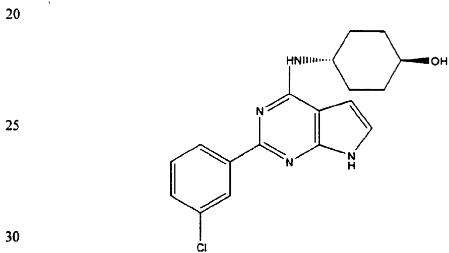
(Compound 1320)
