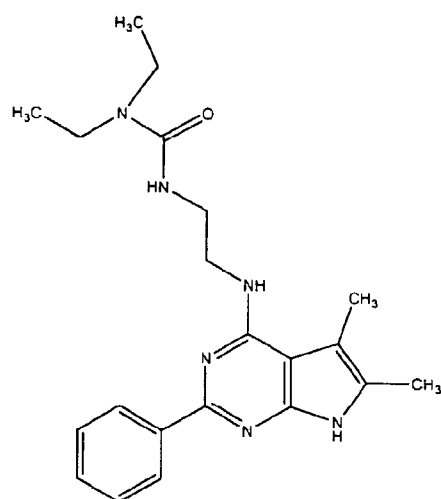
(Compound 1701)
