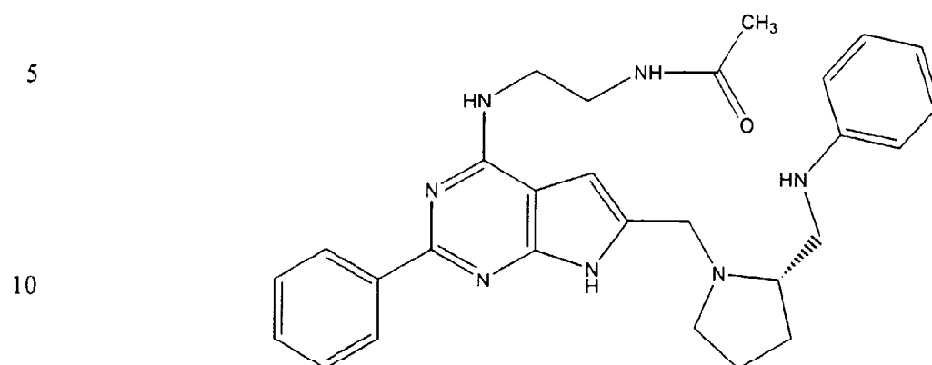
(Compound 1713)
