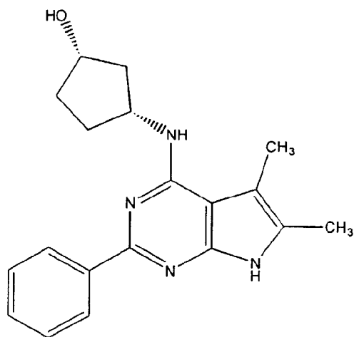
(Compound 609)
