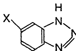
Chemical formula 1
