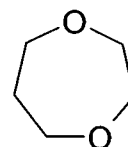
1,4-dioxepanyl
