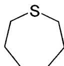
thiepanyl
