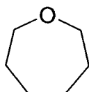
oxepanyl
