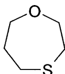
1,4-oxathiepanyl
