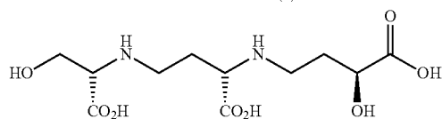
Serine-based analog of Avenic Acid (2)
