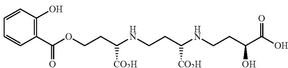
salicylic acid conjugated to avenic acid
