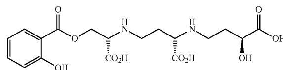
salicylic acid conjugated to serine analog of avenic acid
