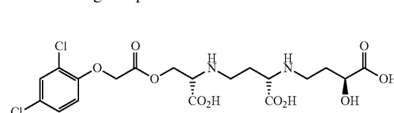
2,4-D conjugated to serine analog of avenic acid
