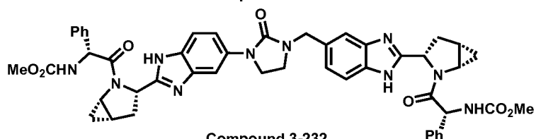
Compound 3-232
