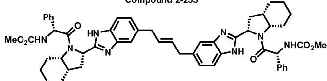
Compound 2-233
