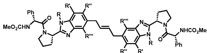
Compounds 2-284 to 2-309
