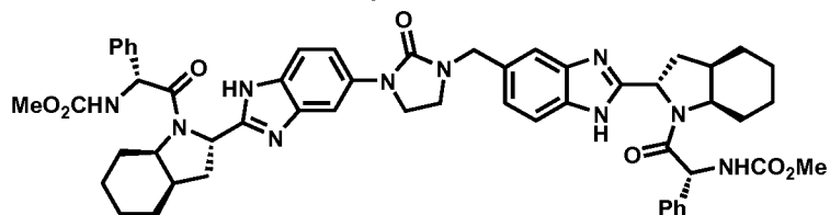
Compound 3-233
