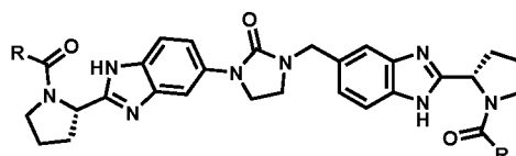
Compounds 3-1 to 3-219
