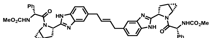
Example 2-232
