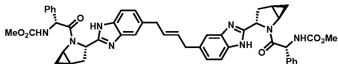
Compound 2-231
