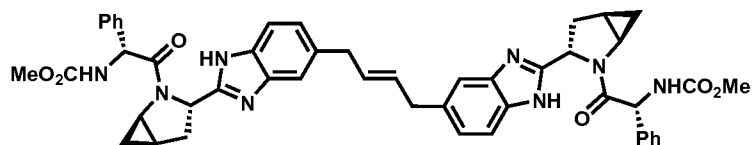
Compound 2-231
