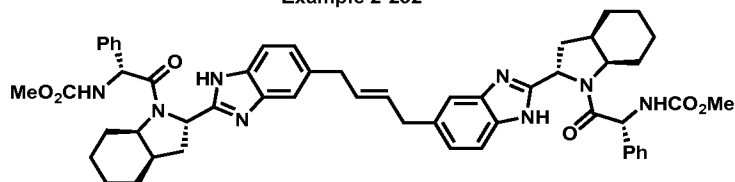
Example 2-233
