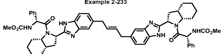
Example 2-233
