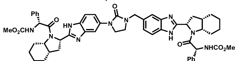
Compound 3-233
