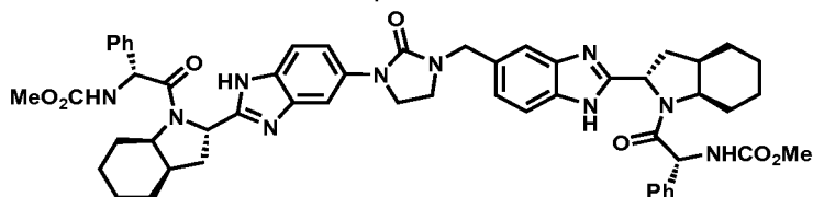
Example 3-233
