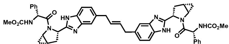
Compound 2-232
