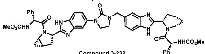
Compound 3-232
