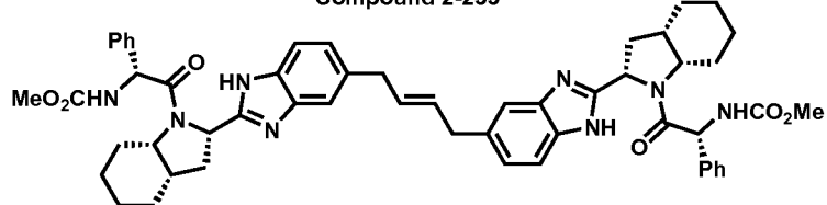
Compound 2-233
