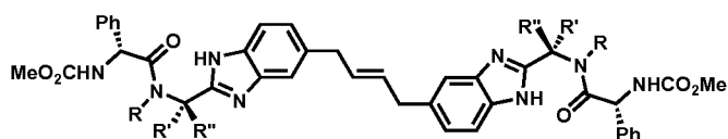
Compounds 2-234 to 2-243
