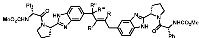
Compounds 2-264 to 2-283
