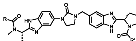
Compounds 3-244 to 3-263
