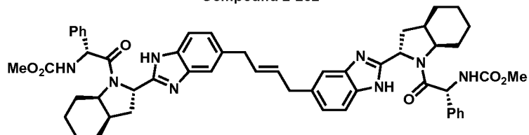
Compound 2-233
