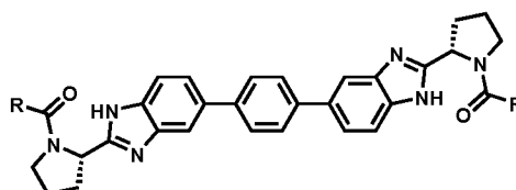
Compounds 1-1 to 1-219
