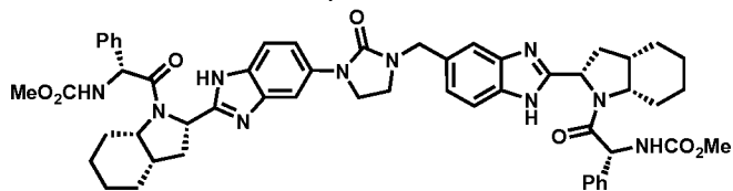
Compound 3-233
