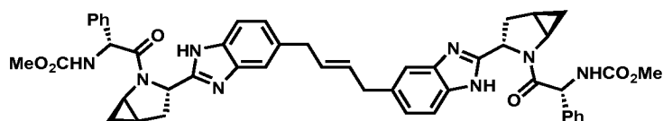
Example 2-231
