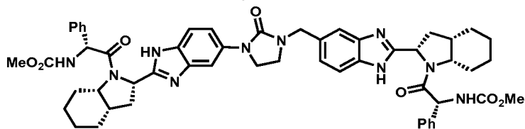
Example 3-233
