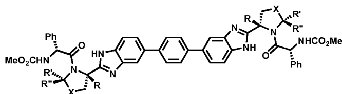
Compounds 1-220 to 1-229
