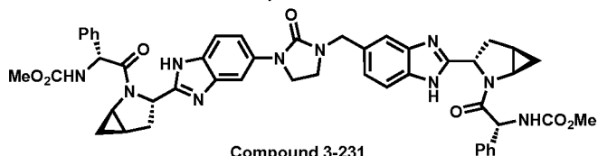
Compound 3-231
