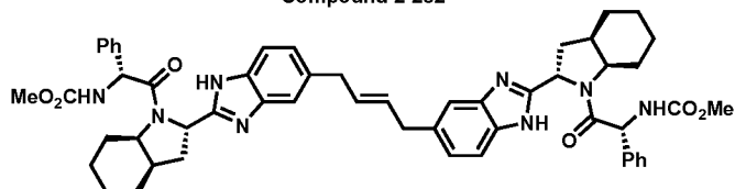
Compound 2-233
