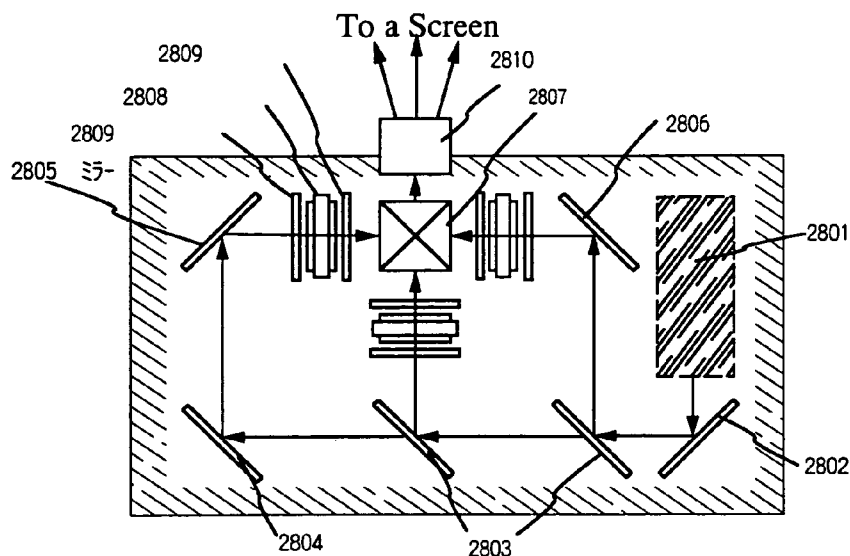
Fig. 18(C) Display Device(3 panel projector)
