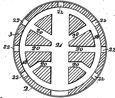
Section G-H Fig. 8
