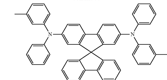
Spiro-TPD
