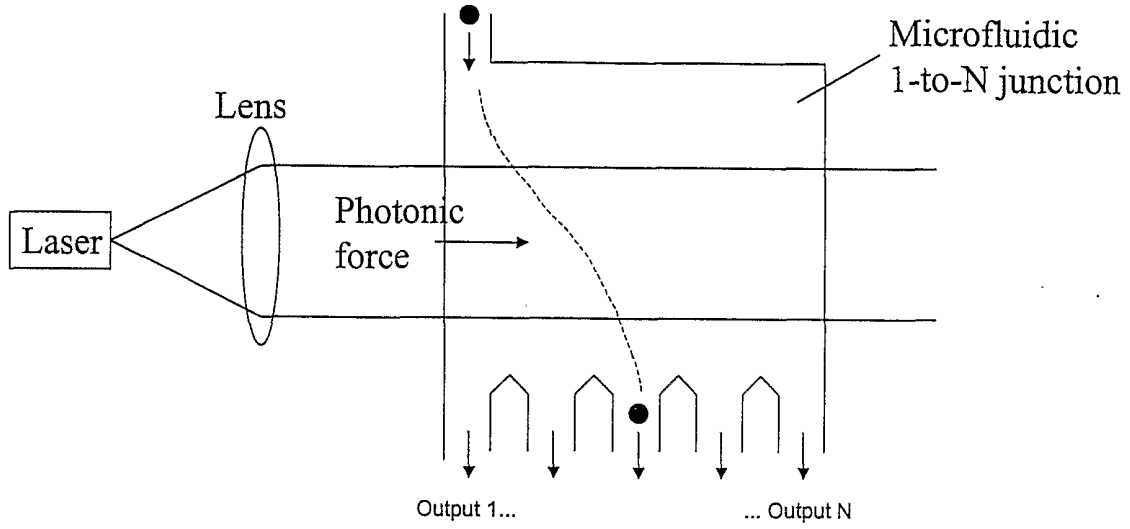
Figure 7c 1-to-N optically-switched microfluidic junction
