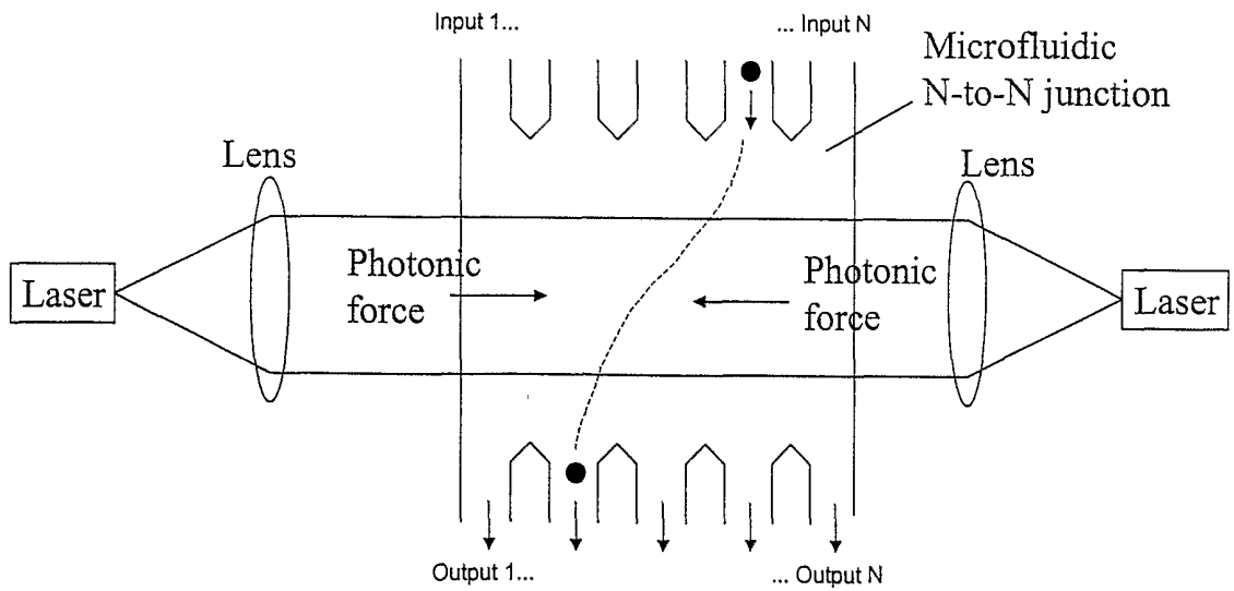
Figure 7d N-to-N optically-switched microfluidic junction
