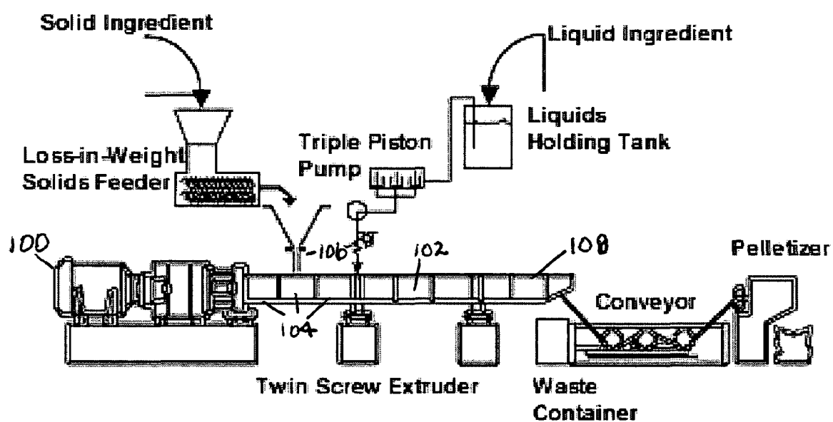
Figure 1. Twin-screw extrusion process used to fabricate continuously graded particle-reinforced polymer composites.
