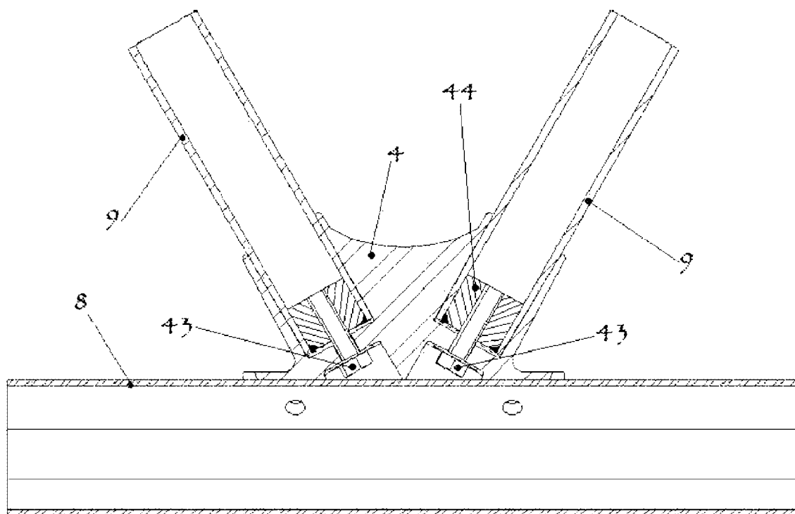
SECTION F-F
