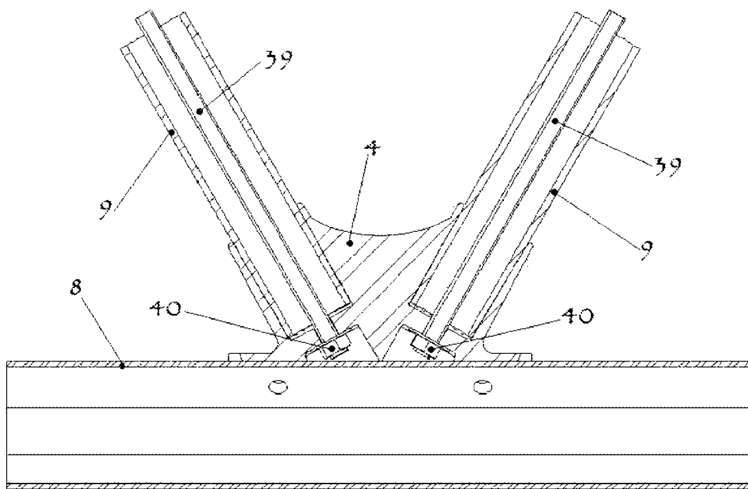
SECTION E-E
