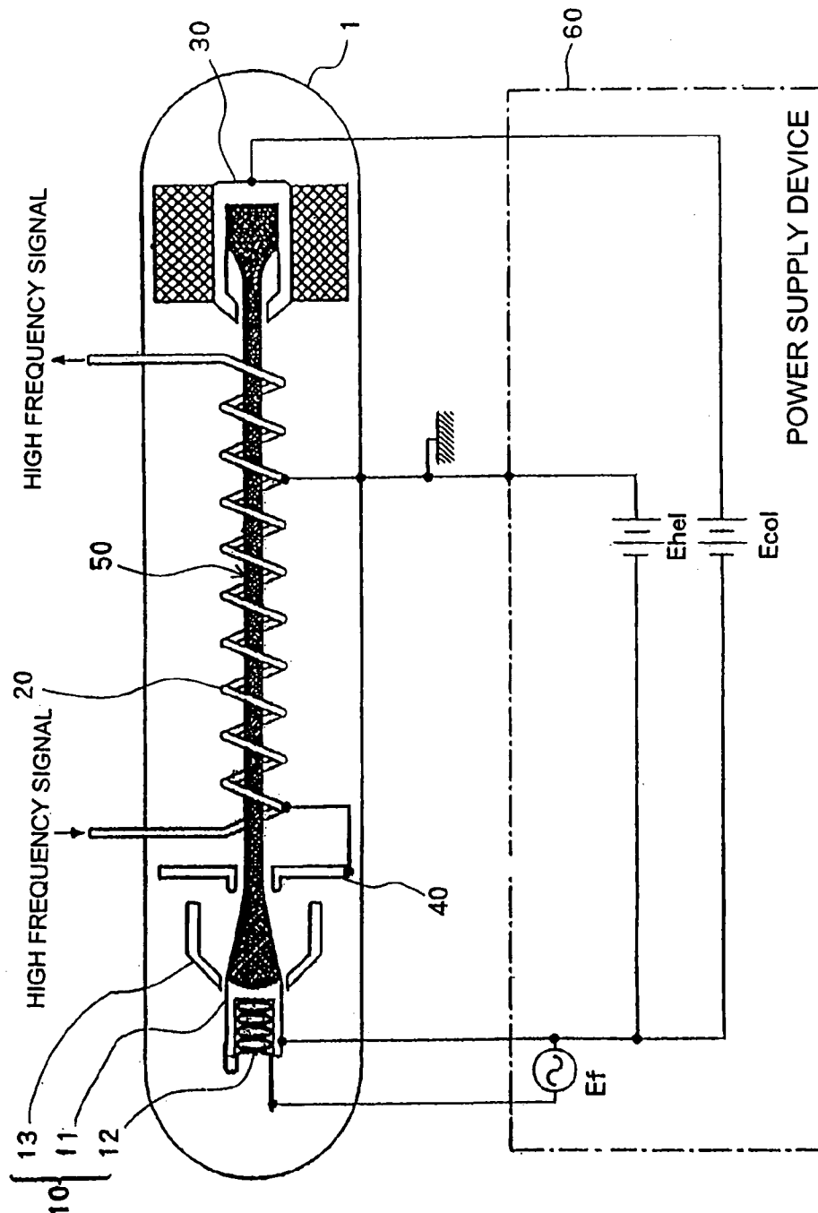
FIG. 1 (PRIOR ART)
