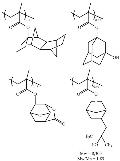
Polymer 2-3
