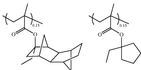
Polymer 2-4
