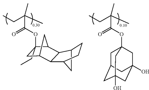
Polymer 2-8
