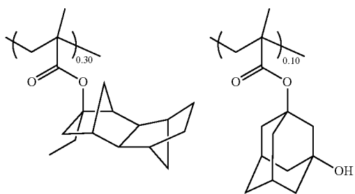
Polymer 2-6
