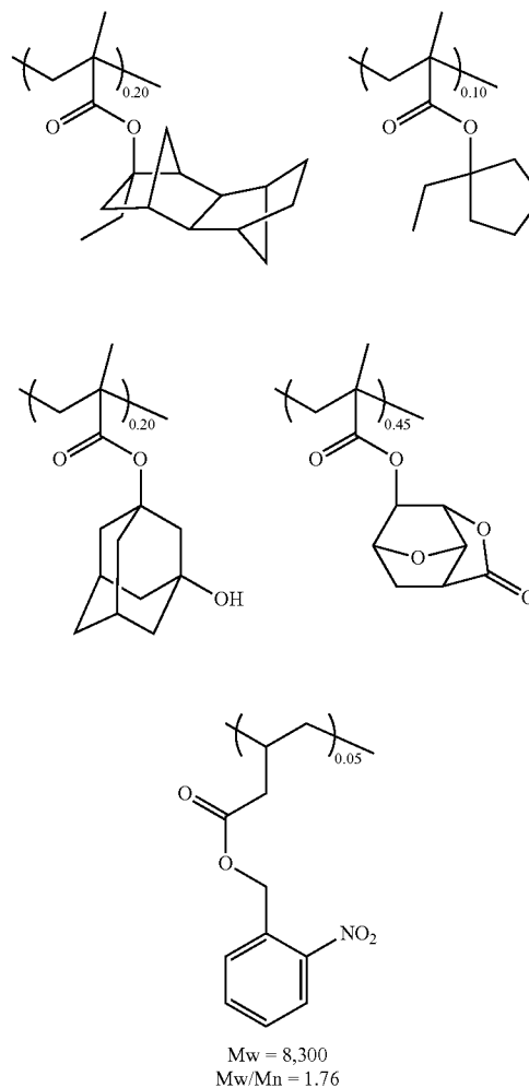
Polymer 1-1
