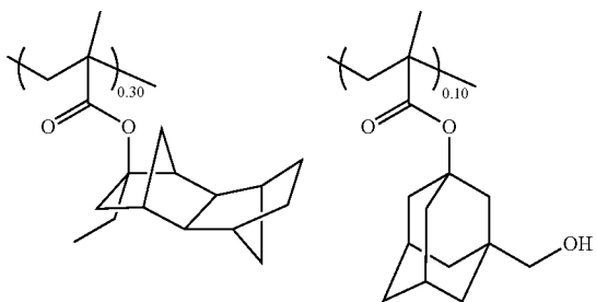
Polymer 2-7
