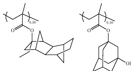
Polymer 2-5
