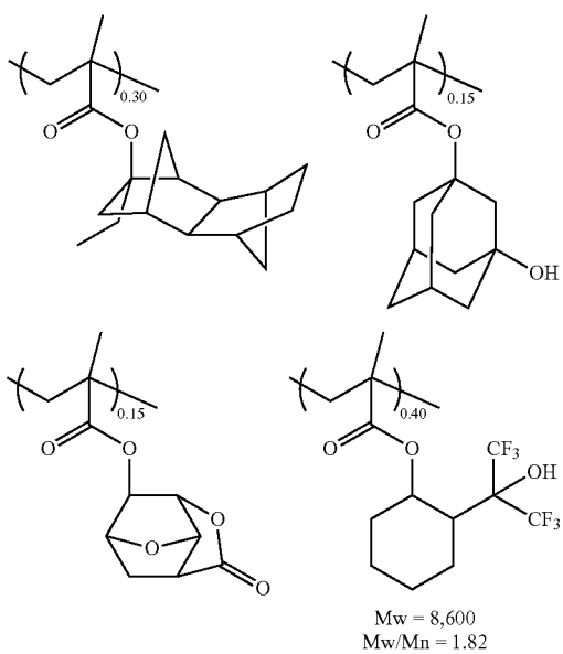
Polymer 2-4
