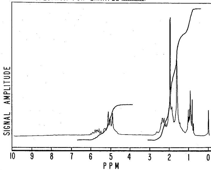
N M N SPECTRUM FOR EXAMPLE XXXIII
