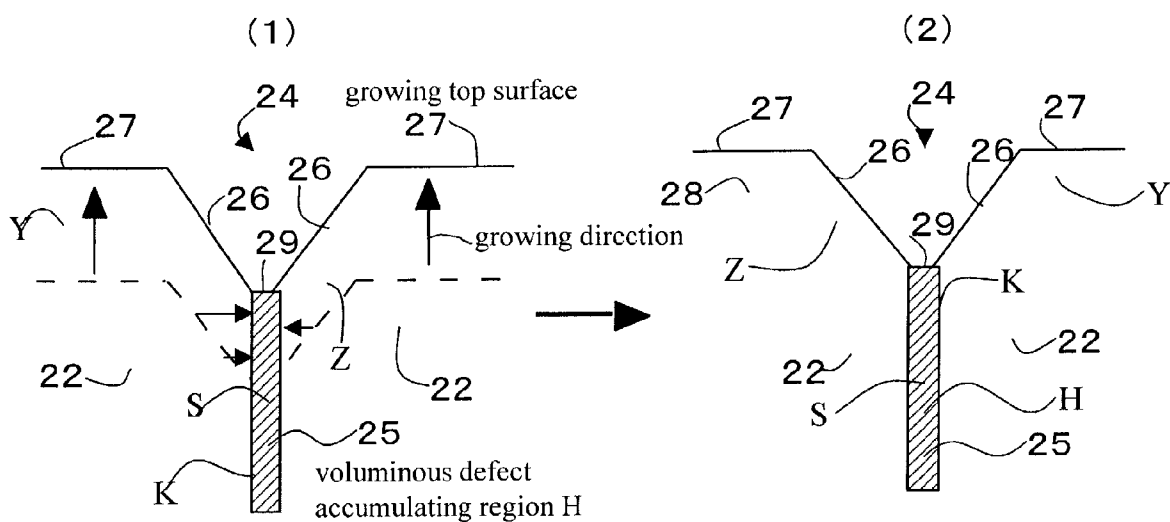
Fig.4 Growing method of the present invention
