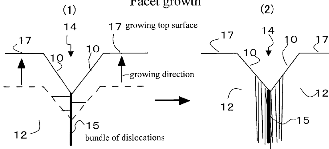
Fig.4 Growing method of the present invention
