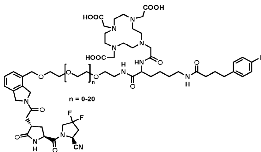
FAP-3024 (with an ether linkage +albumin binder)
