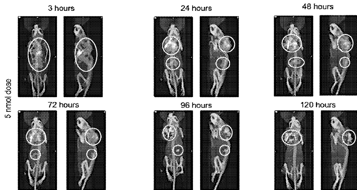
Fig. 7A SPECT/CT of ^{111}\text{In} -FAP-3001 in 4T1 tumors
