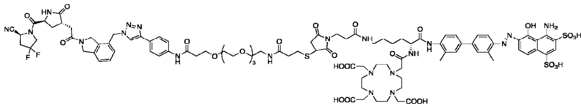
FAP-3011 (with phenyl ring spacer, Evans Blue albumin-binder)
