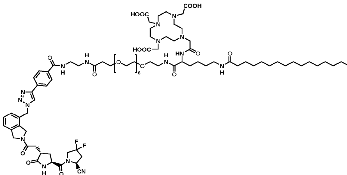
FAP-3028 with fatty acid albumin-binder (triazole +phenyl)
