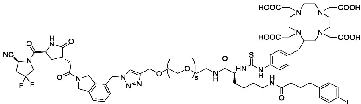
FAP-3005 (with SCN-Bn-DOTA)
