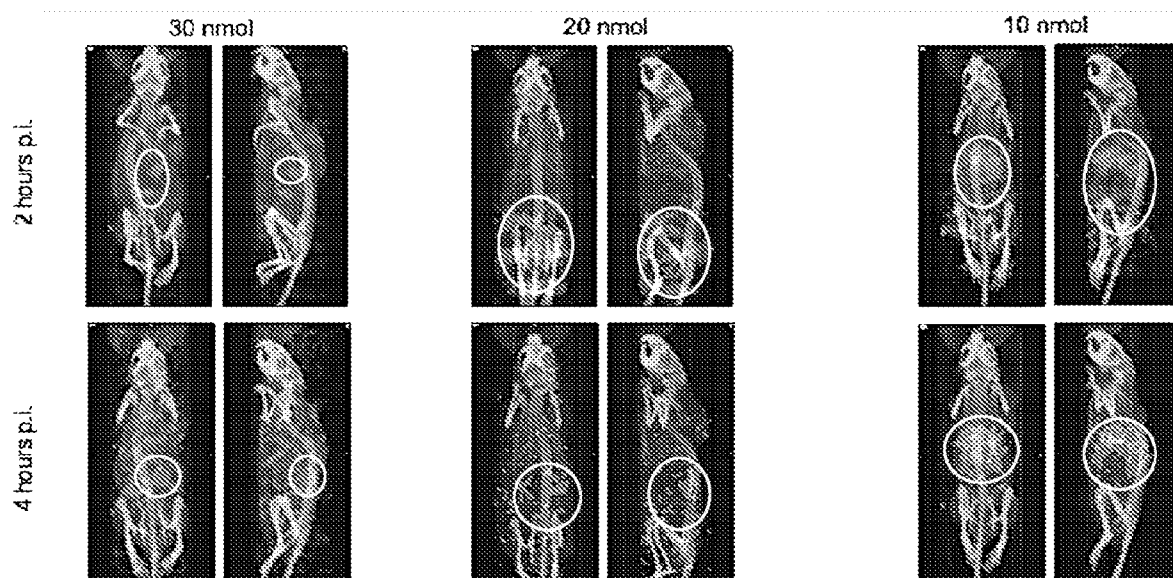
Fig. 6A SPECT/CT of ^{111}\text{In} - FAP-3000 in 4T1 tumors
