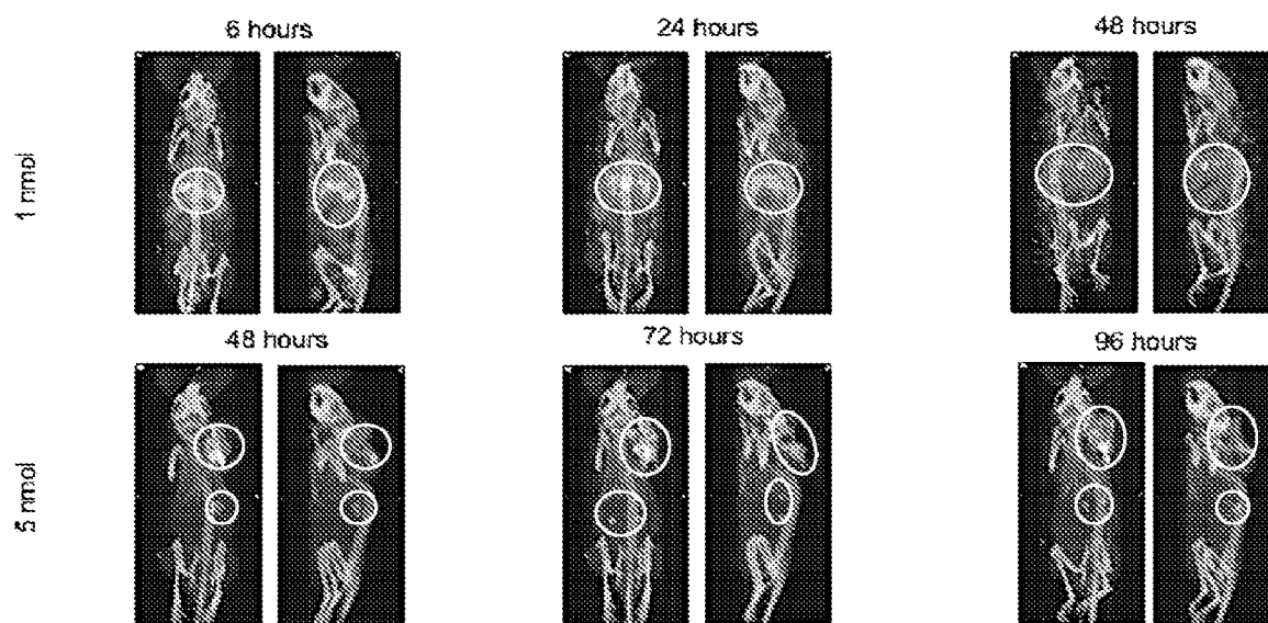
Fig. 5B SPECT/CT of ^{111}\text{In} -FAP-3001 in HT29 tumors
