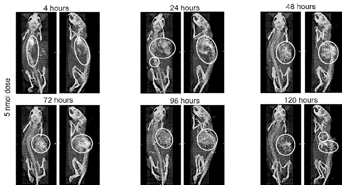
Fig. 7B SPECT/CT of ^{111}\text{In} -FAP-3001 in KB tumors
