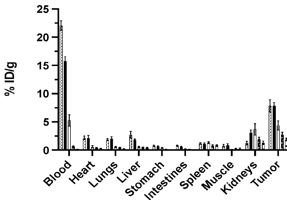
Fig. 8B Biodistribution of ^{111}\text{In} -FAP-3001
