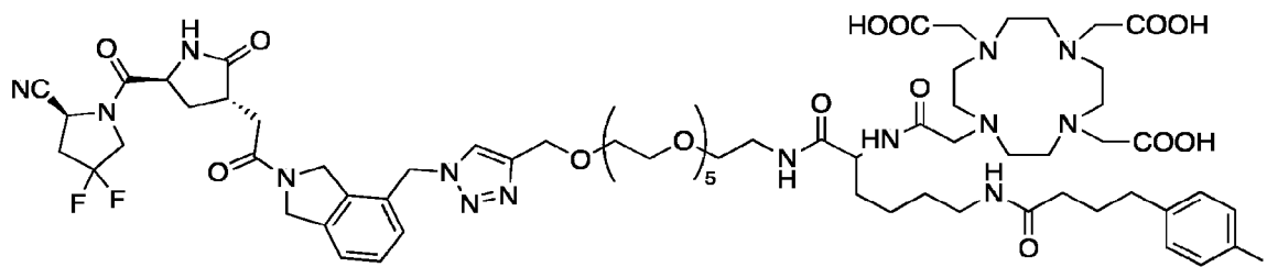
FAP-3001 (with iodobenzene albumin-binder)
