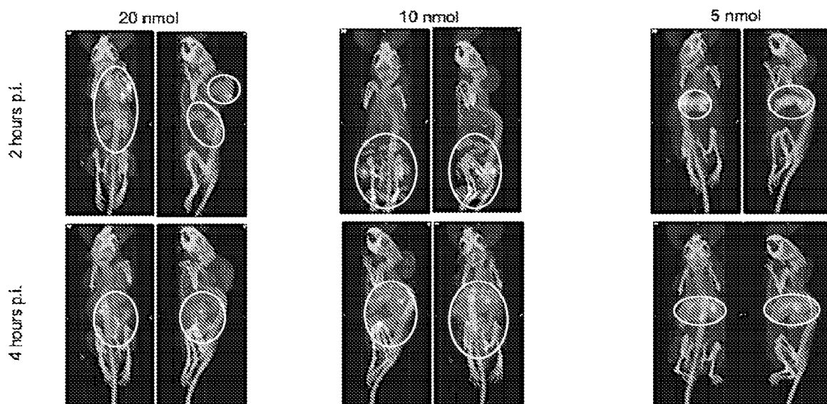
Fig. 5A SPECT/CT of ^{111}\text{In} -FAP-3000 in HT29 tumors
