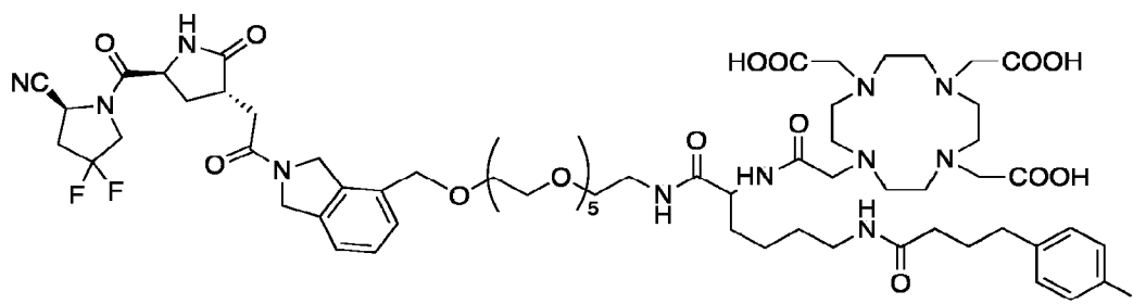
FAP-3012 (with an ether linkage that does not require click chemistry)
