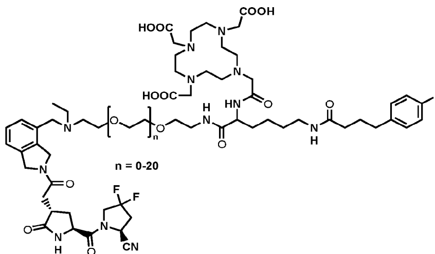
FAP-3026 (with tertiary amine linkage +albumin binder)
