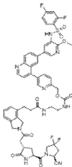
FAP5-Carbamate-PI3Ki
