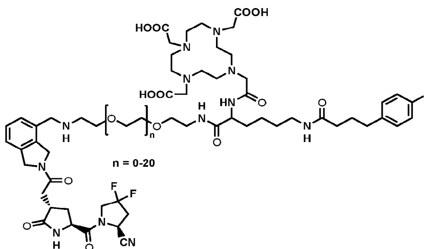
FAP-3025 (with an amine linkage +albumin binder)
