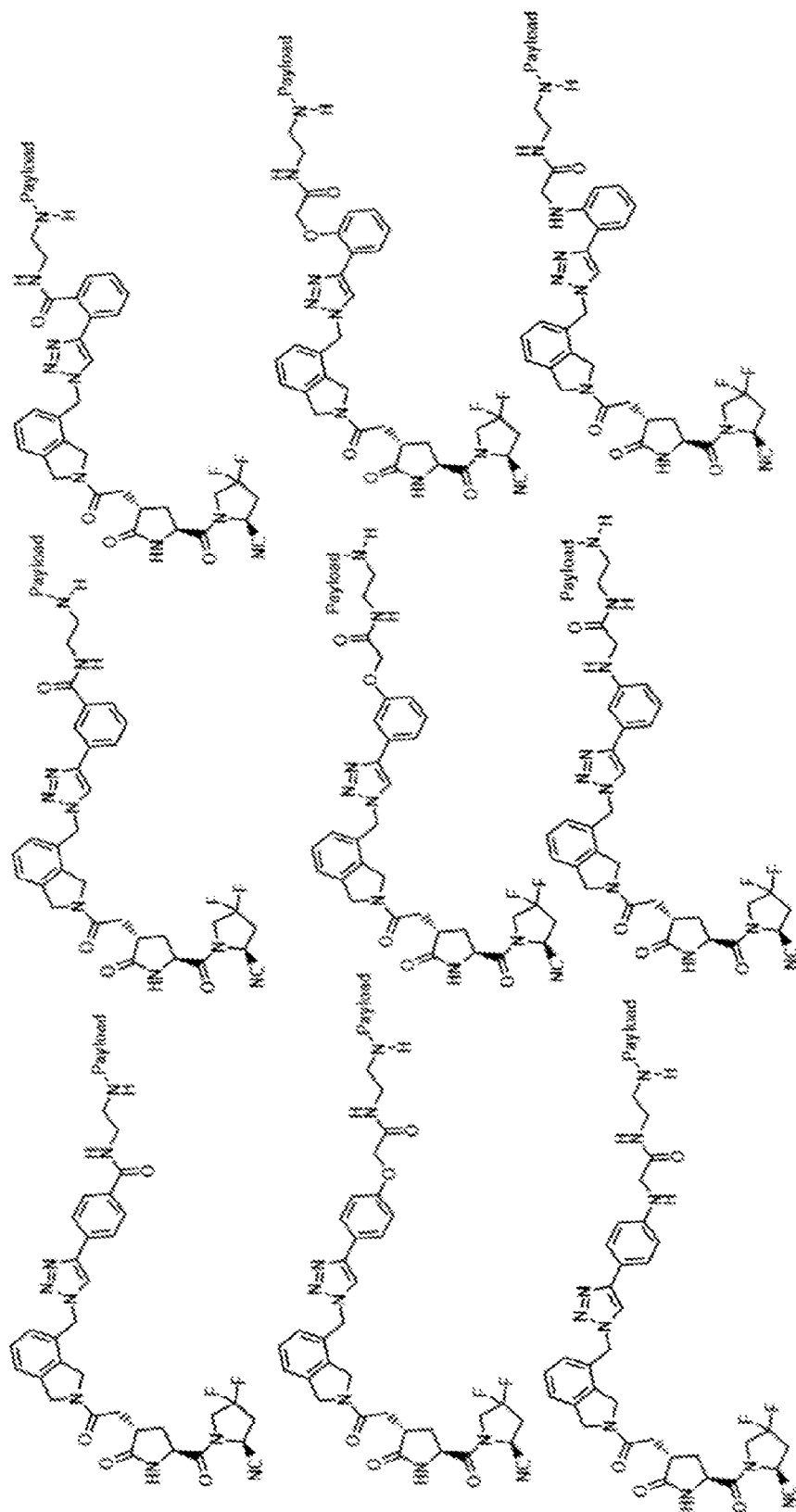
FAP6 Analogs (no linker)
