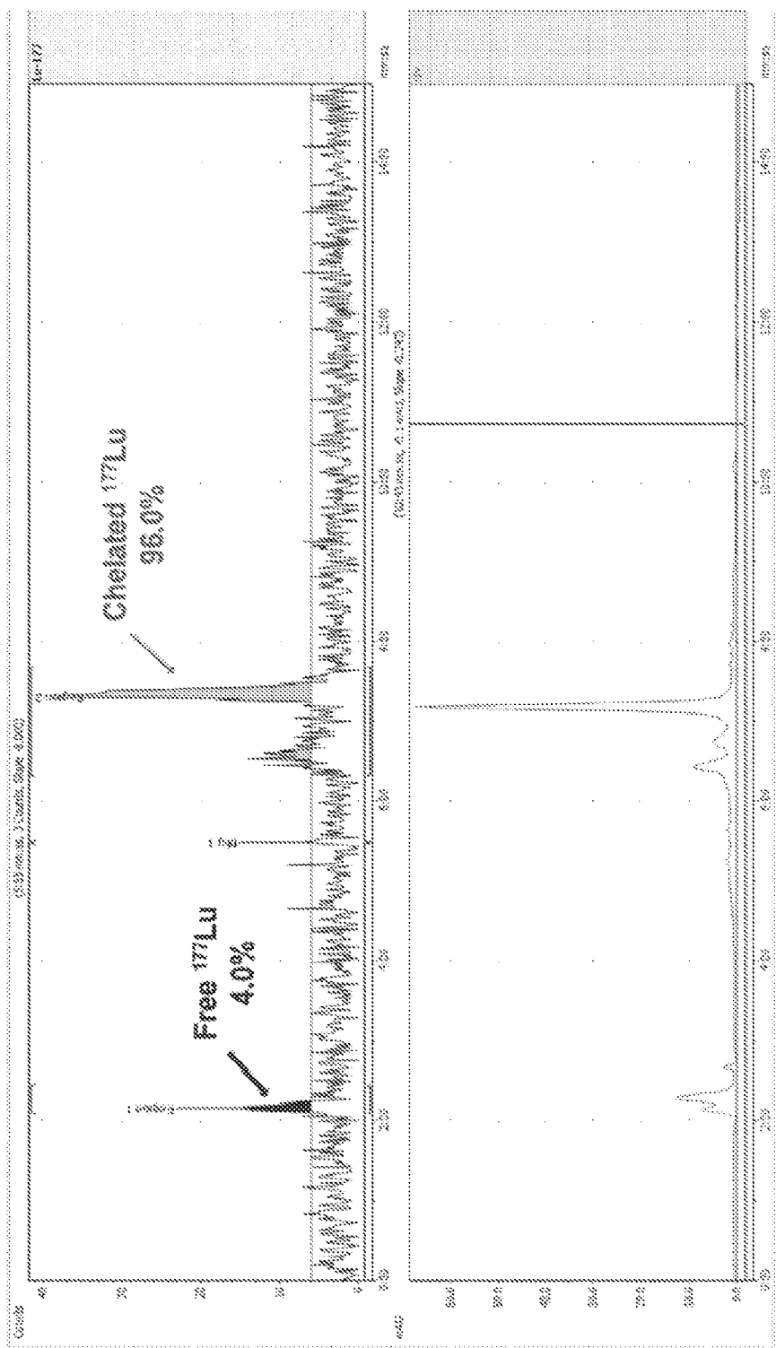
Fig. 3B ^{177}\text{Lu} radiolabeling of FAP-3000
