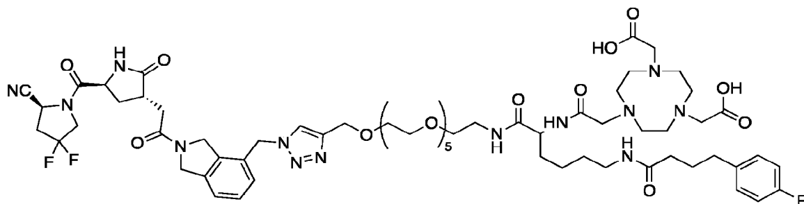
FAP-3002 (with NOTA, fluorobenzene albumin-binder)
