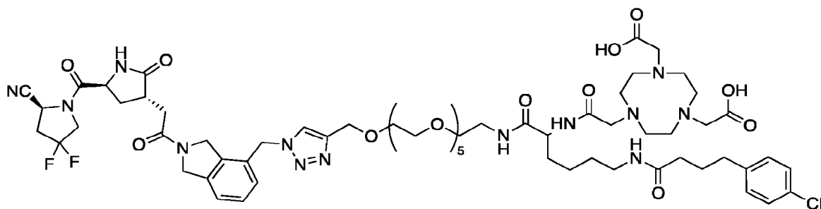
FAP-3003 (with NOTA, chlorobenzene albumin-binder)
