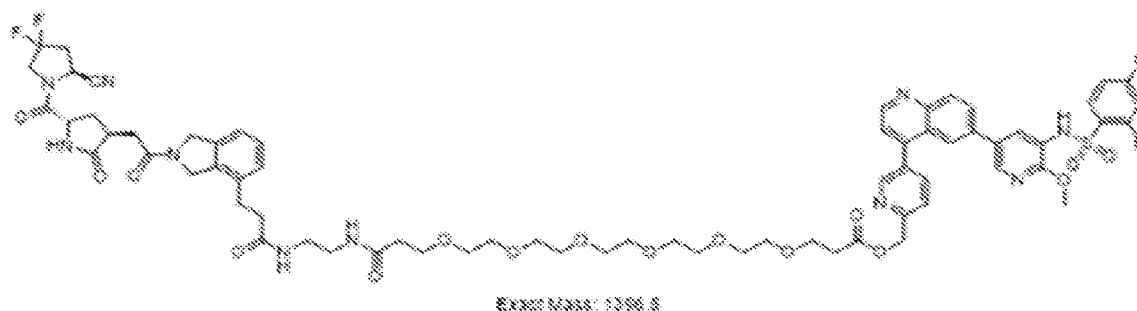
FAPS-Ester-PI3Ki
