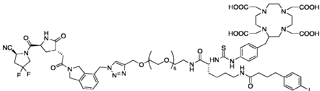
FAP-3006 (with D-Lysine, SCN-Bn-DOTA)
