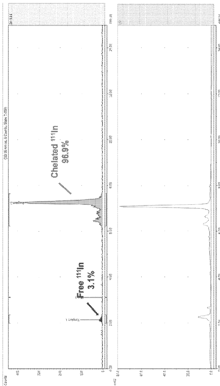
Fig. 3A In-111 radiolabeling of FAP-3000
