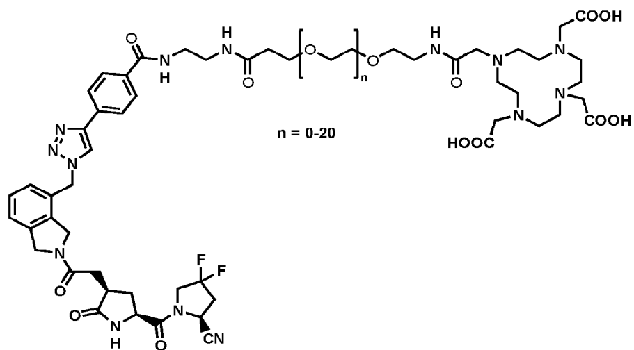
FAP-3018 (with Cis stereochemistry at pyrrolidine ring)
