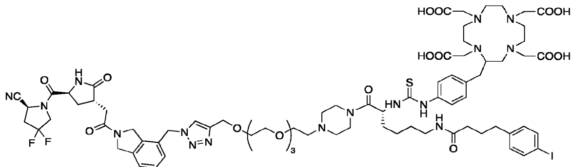
FAP-3007 (with piperazine, D-Lysine, SCN-Bn-DOTA)
