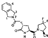
FAP Inhibitor 1
