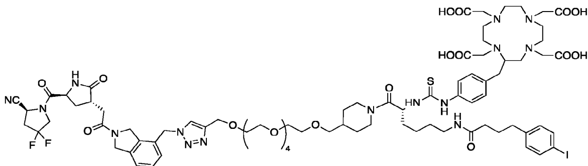
FAP-3009 (with piperidine, D-Lysine, SCN-Bn-DOTA)
