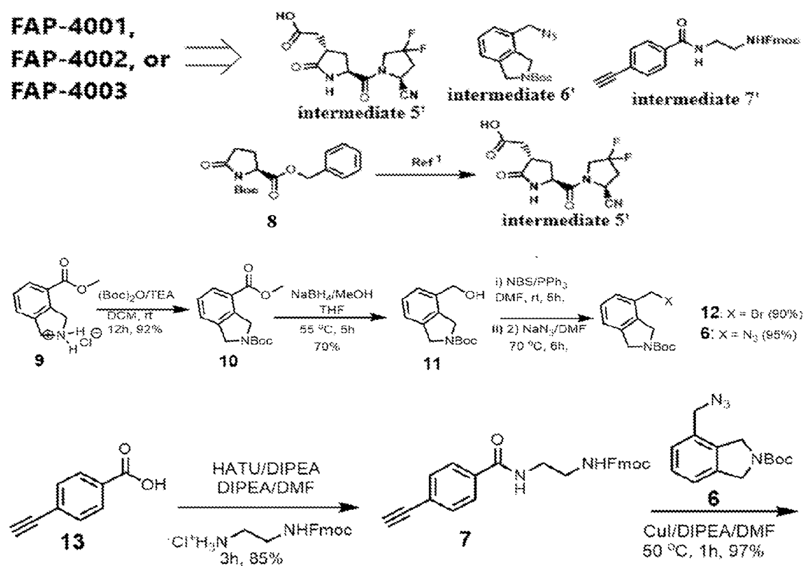
Scheme 2
