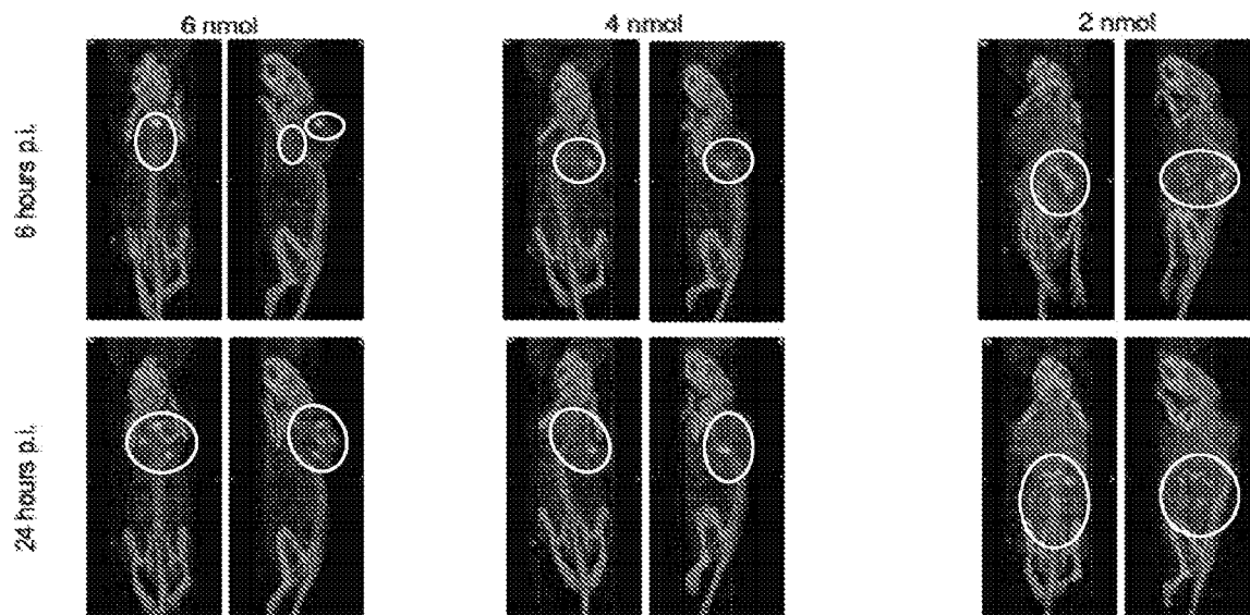
Fig. 6B SPECT/CT of ^{111}\text{In} - FAP-3001 in 4T1 tumors
