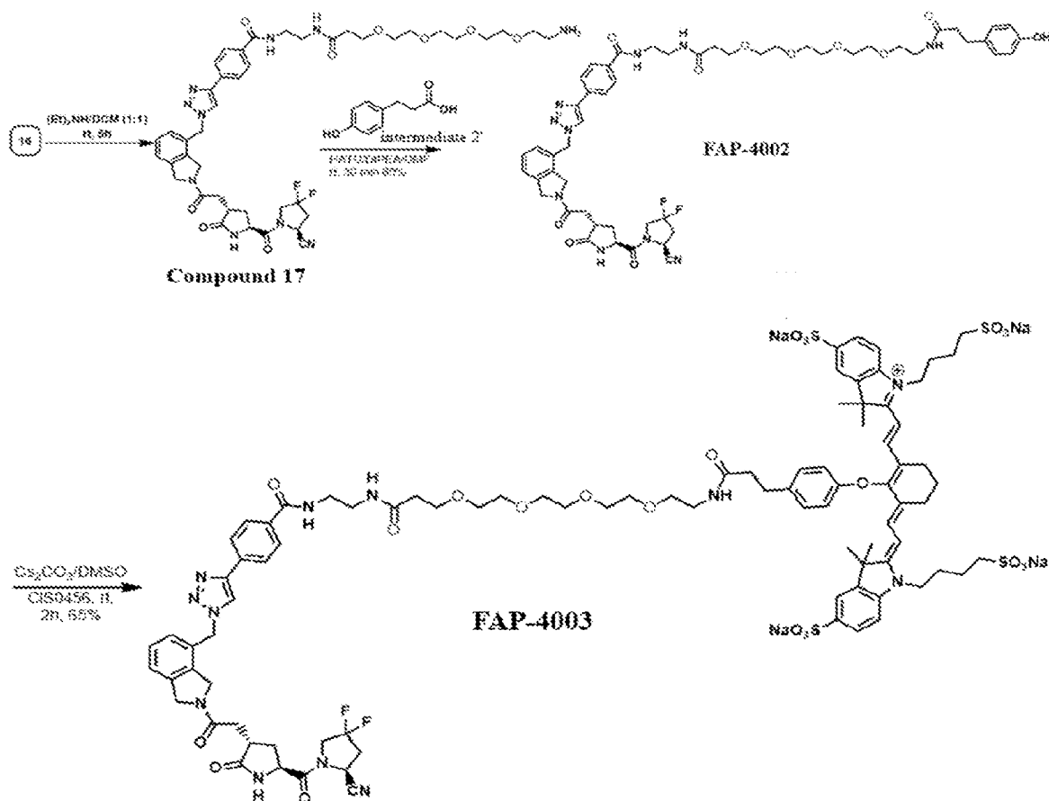
Scheme 3
