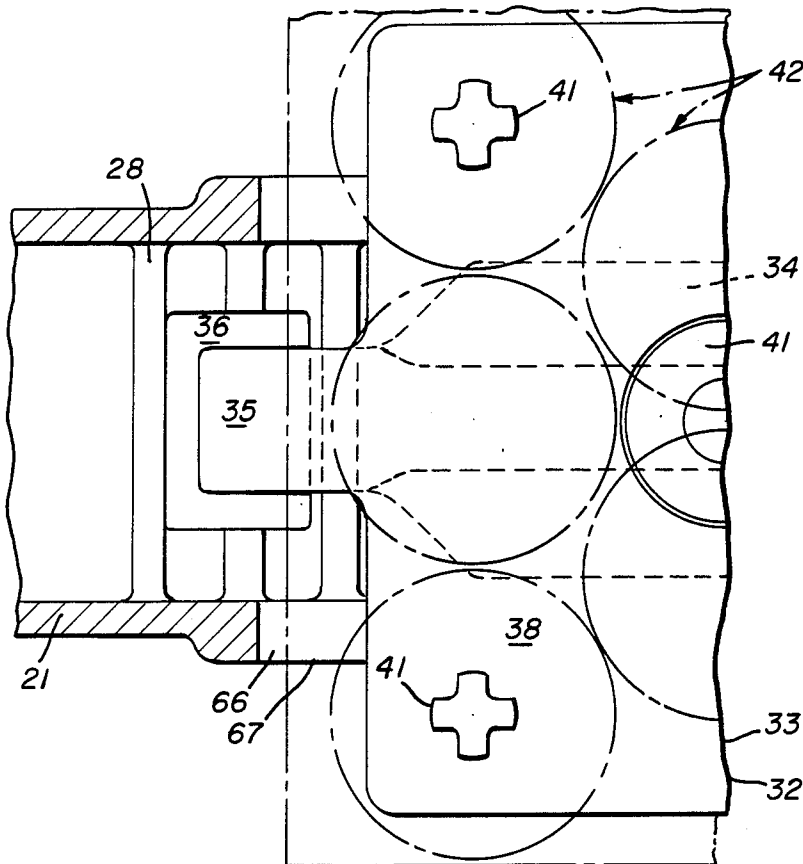
FIG. 6 PRIOR ART
