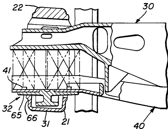
FIG. 8 PRIOR ART
