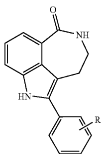
Tricyclic lactam indoles T13: R = 4'-F R = H R = 3-NH 2 R = 2-OH
