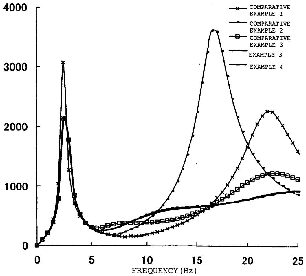
FIG. 56 VARIATIONS IN LONGITUDINAL FORCE OF TIRE (N/Hz)
