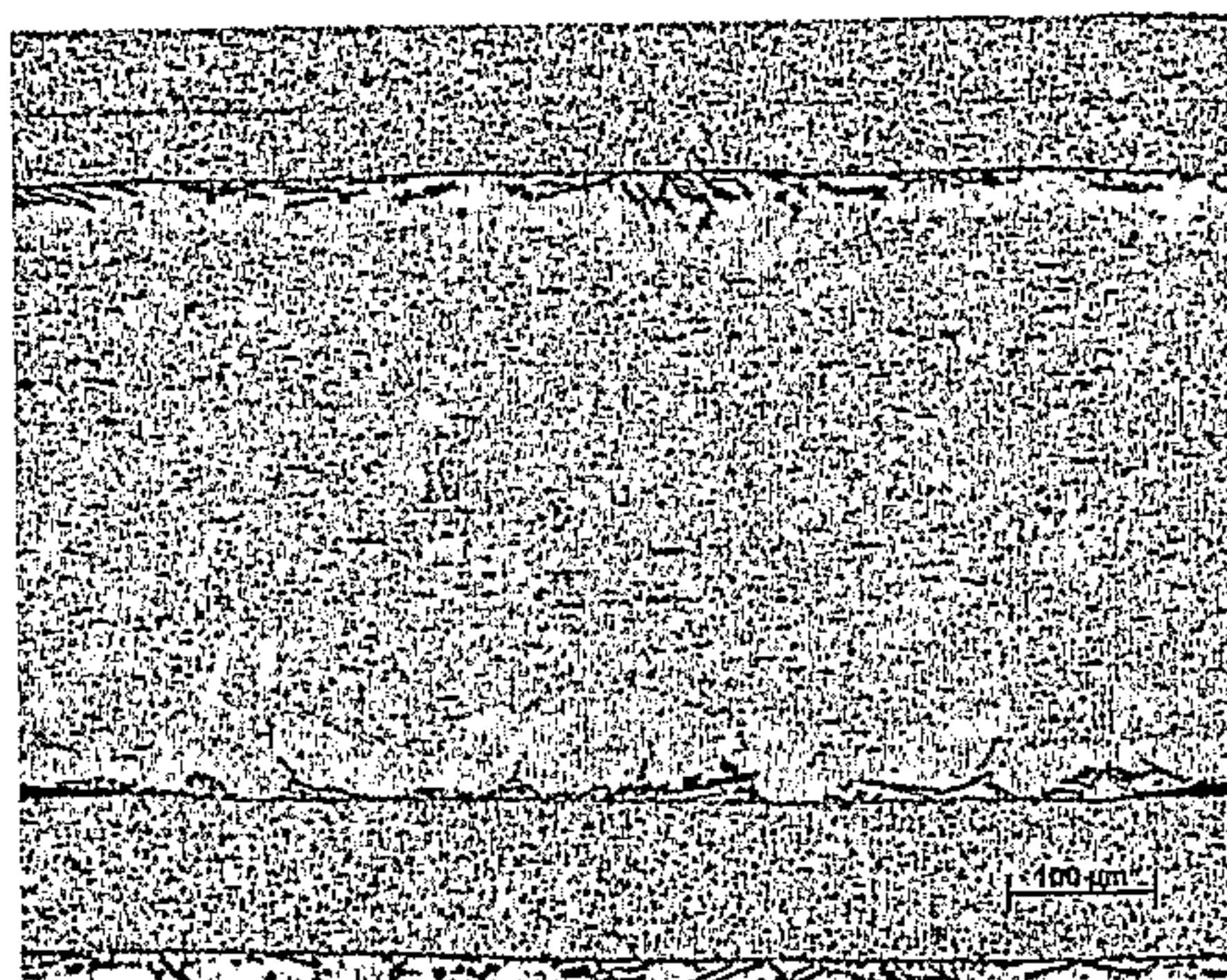
8% Stretch FIG. 7f Prior Art
