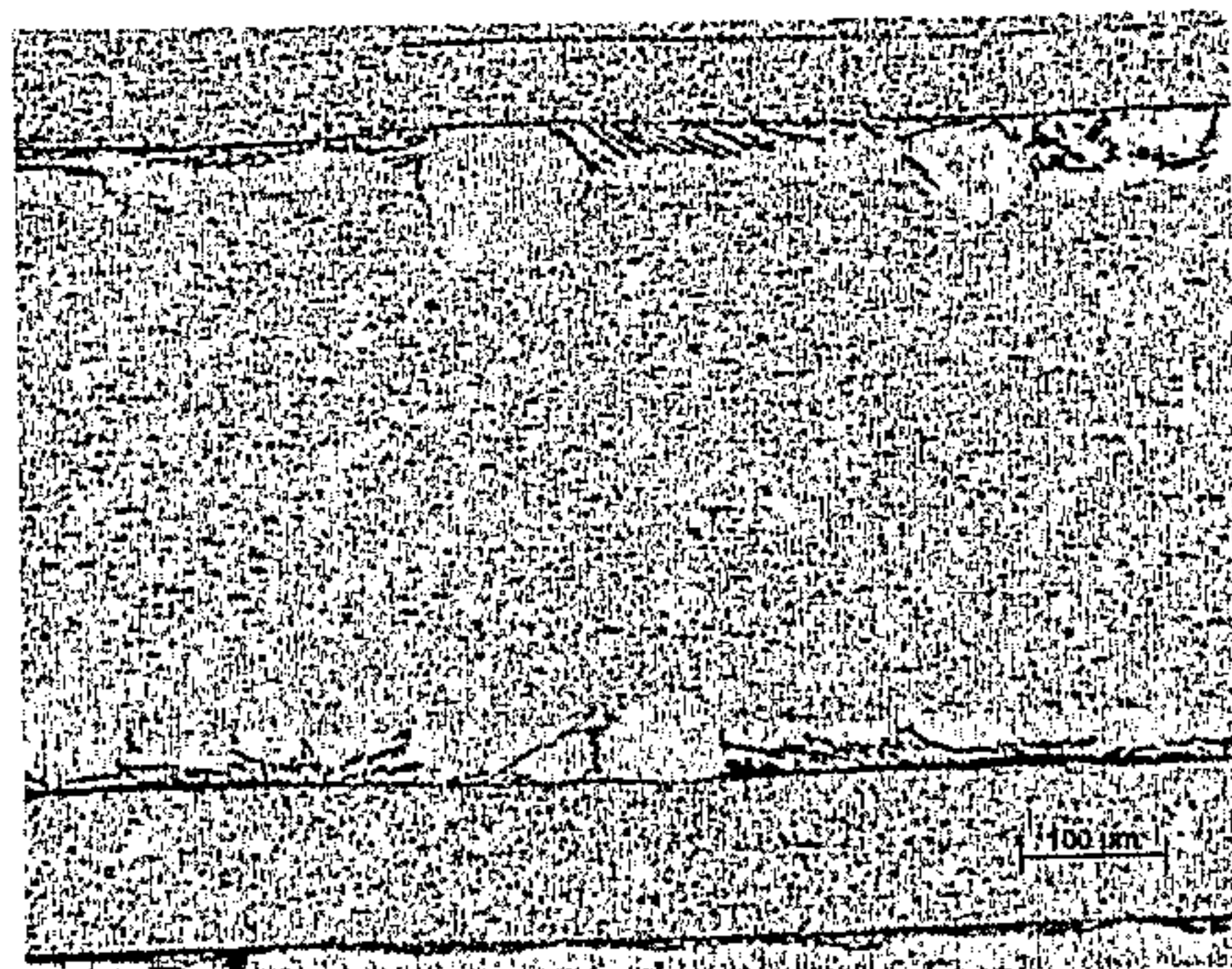
2% Stretch FIG. 7c Prior Art
