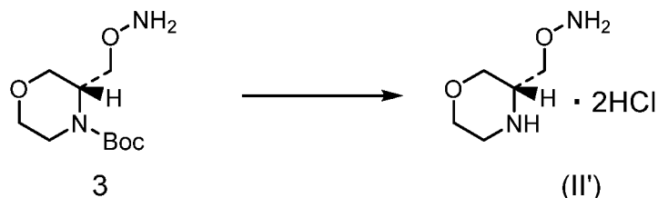
[Chemical Formula 28]
