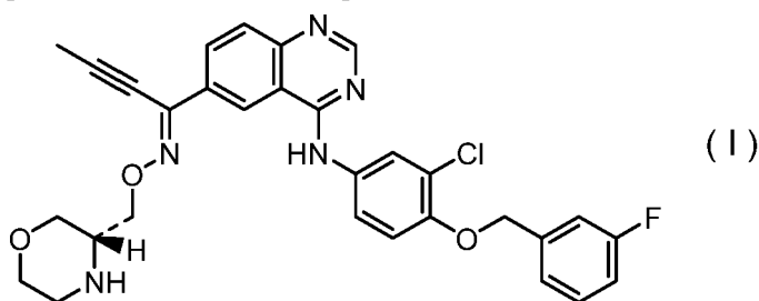
[Chemical Formula 12]
