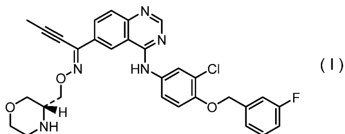
[Chemical Formula 2]
