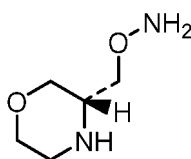
[Chemical Formula 21]
