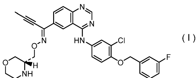
[Chemical Formula 2]
