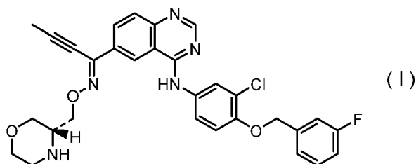
[Chemical Formula 13]
