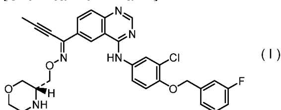
[Chemical Formula 11]
