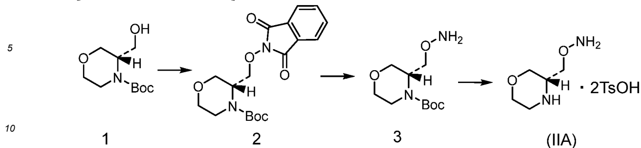
[Chemical Formula 27]
