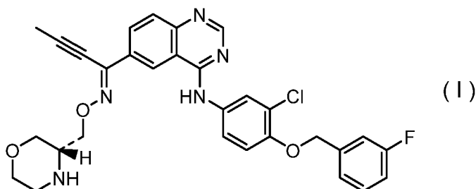
[Chemical Formula 22]
