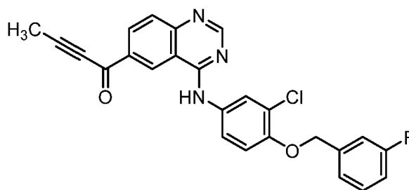
[Chemical Formula 20]
