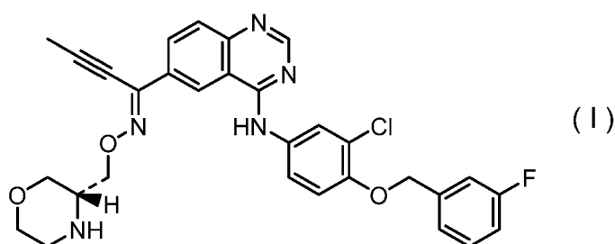
[Chemical Formula 2]
