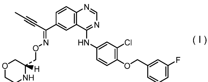
[Chemical Formula 2]
