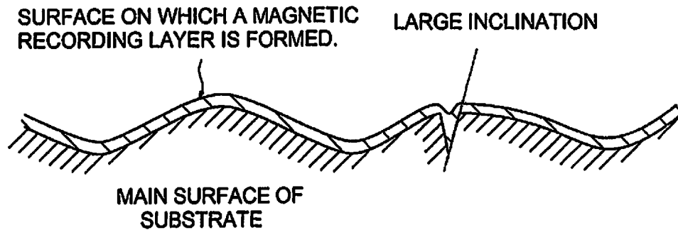
FIG. 2B THICKNESS BETWEEN MAGNETIC RECORDING LAYER AND SUBSTRATE IS SMALL.
