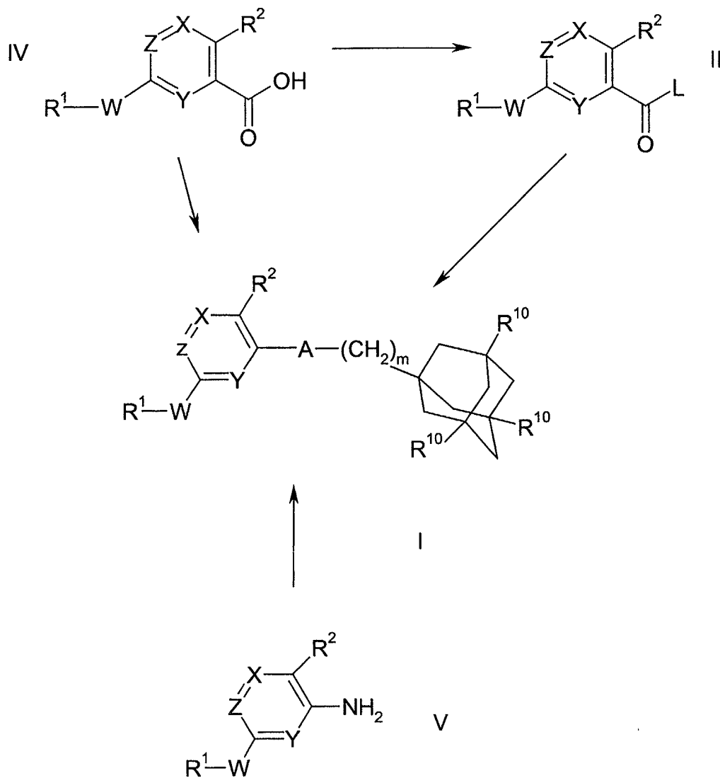
Scheme 1
