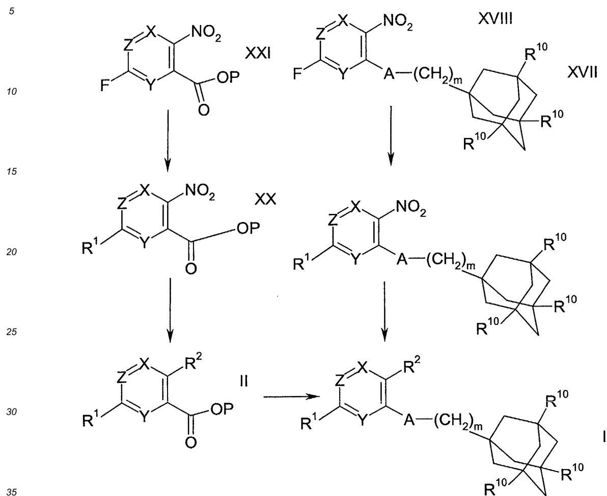
Scheme 5
