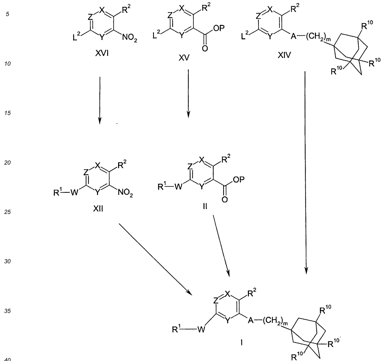
Scheme 4
