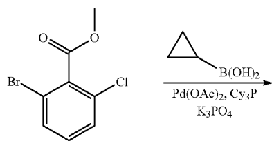
Scheme i-9
