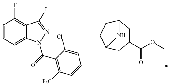
Scheme G
