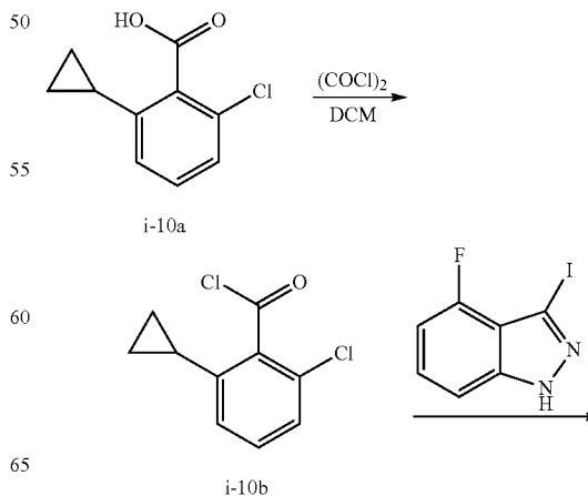
Scheme i-10
