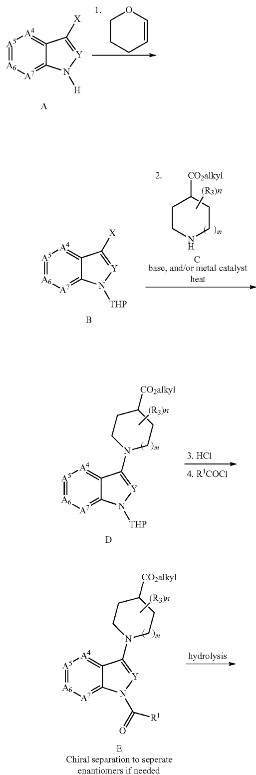
Scheme 2
