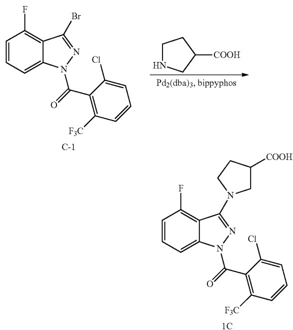
Scheme C
