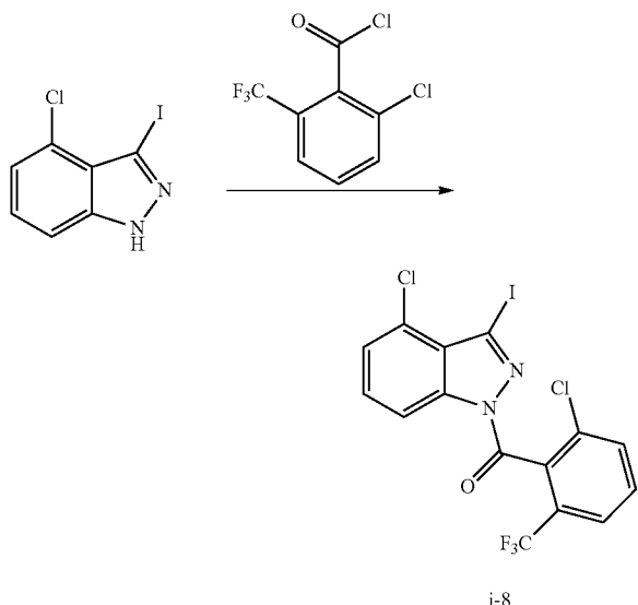
Scheme i-8
