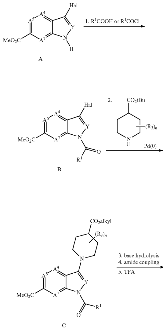
SCHEME 3
