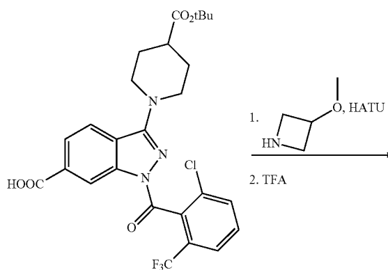
Scheme N
