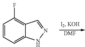
Scheme i-7
