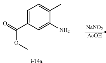
Scheme i-14
