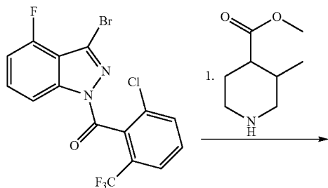
Scheme F
