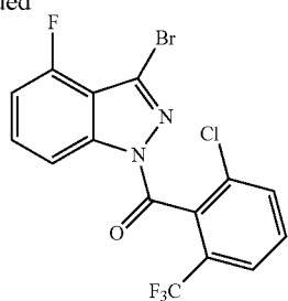
i-12
