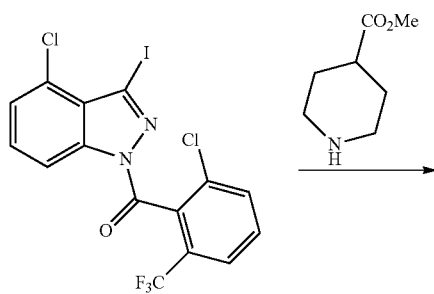
Scheme D
