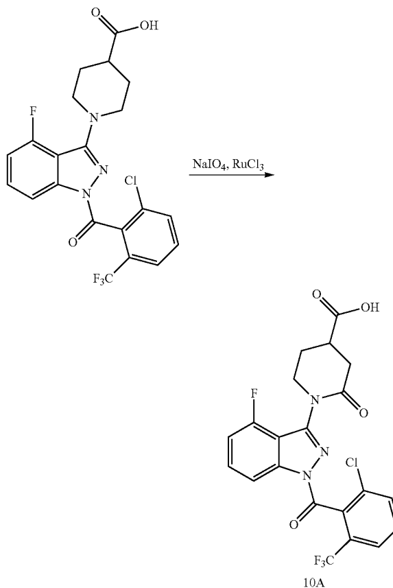
Scheme L
