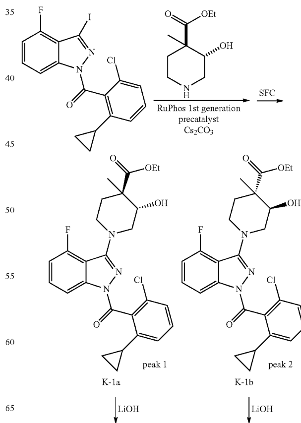
Scheme K
