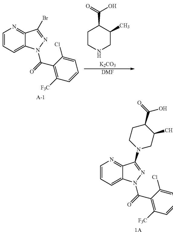
Scheme A
