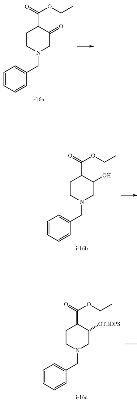
Scheme i-16
