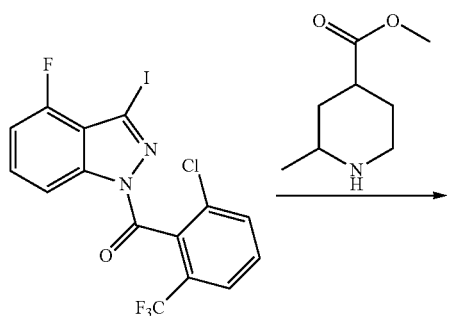
Scheme M
