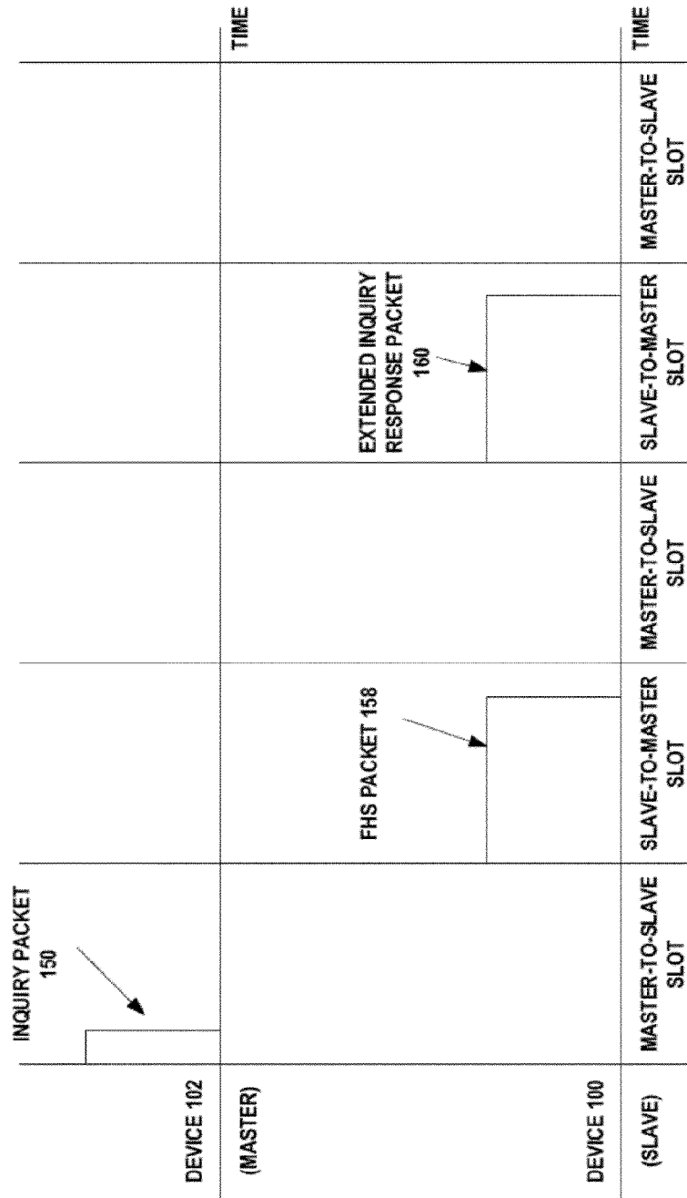
FIG. 2B DEVICE DISCOVERY PHASE 200
