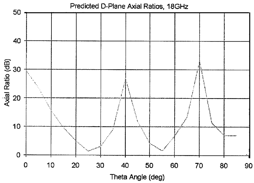
Fig. 10b (End-loaded design)
